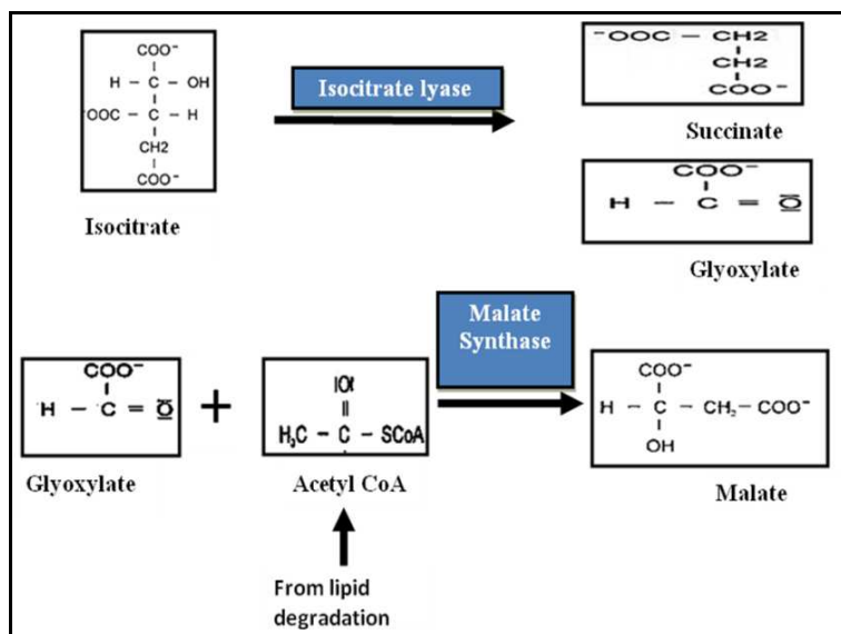
Fig. 2. Reaction scheme of glyoxylate shunt.
