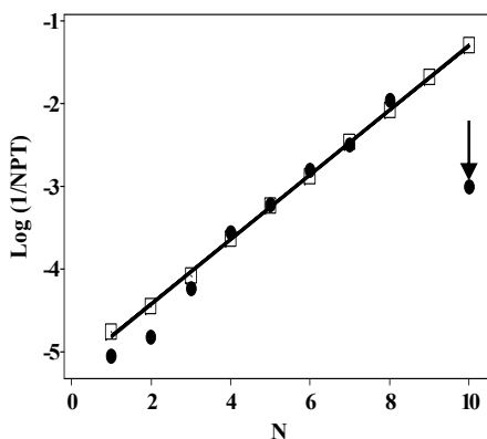
Fig. 5. A plot of \log(1/\text{NPT}) for n-alkyl acetates against N, the number of carbon atoms in the n-alkyl group; ● observed values, □ calculated values from Eqn 36.
