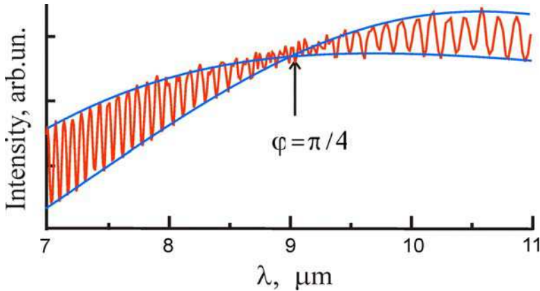
Fig. 12. Experimental spectra of thermal radiation of a free plane-parallel n-InAs plate and envelope lines (blue lines), d = 80 \mu\text{m} . H = 18 \text{ kG} ; temperature is 355K.
