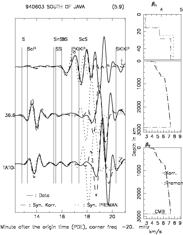
Fig. 12. The seismogram fitting of South Java trench C060394F earthquake in TATO.
