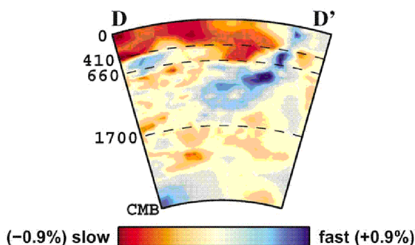
Fig. 1. Depth cross section DD' in front area of subduction zone area in Java-Sumatra, as revealed by P travel-time tomography using ISC data (Romanowicz, 2003)
