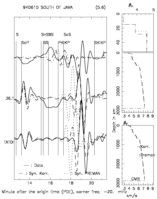
Fig. 13. The seismogram fitting of South Java trench B061594F earthquake in TATO.
