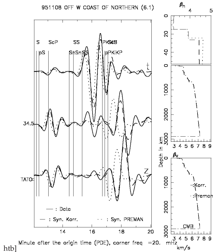
Fig. 5. The seismogram fitting of North Sumatra C110895A earthquake in TATO.
