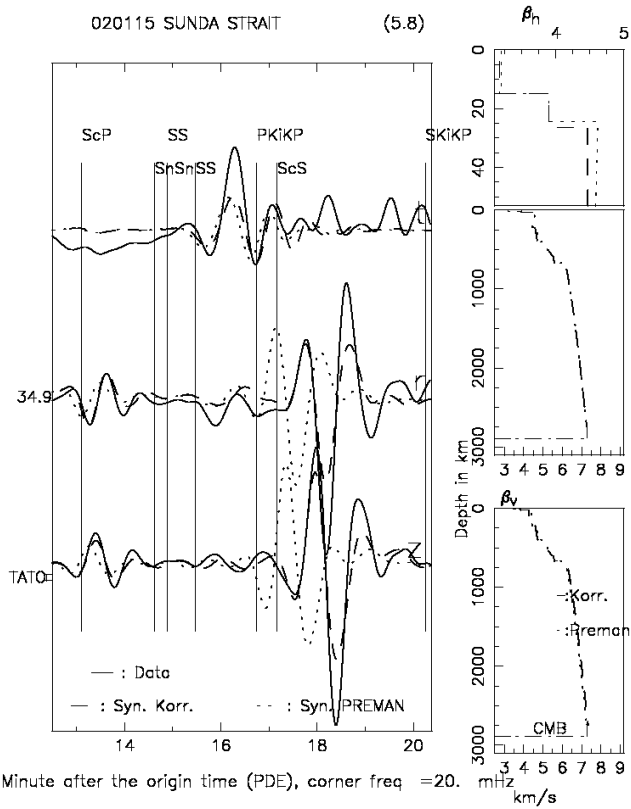
Fig. 11. The seismogram fitting of Sunda Strait C011502D earthquake in TATO.
