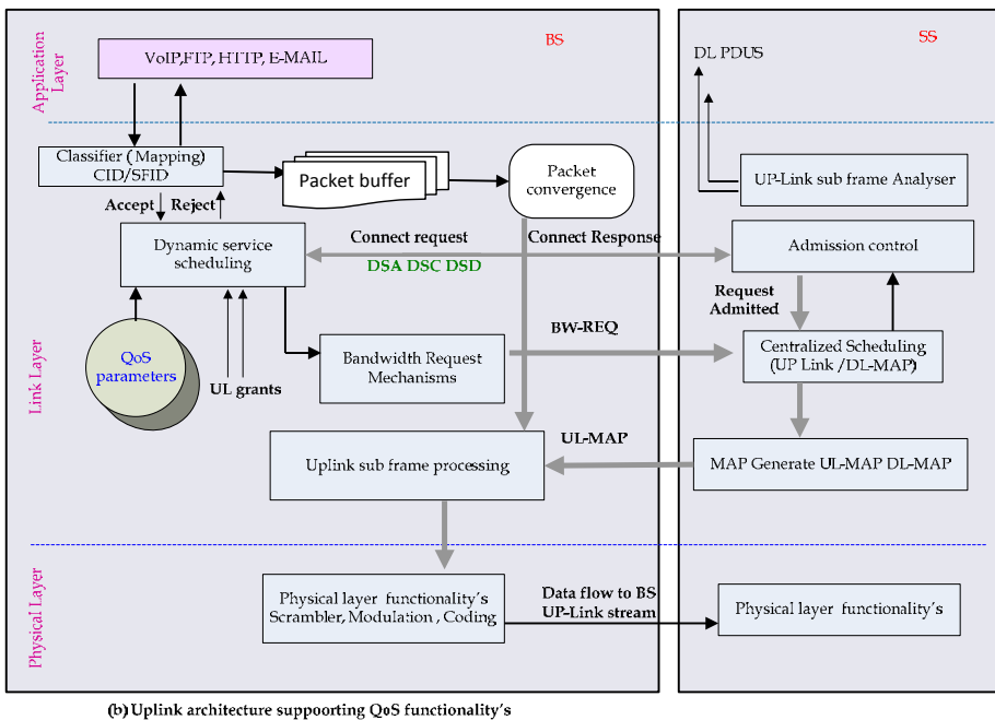
Fig. 3. QoS support for multimedia services in IEEE 802.16
