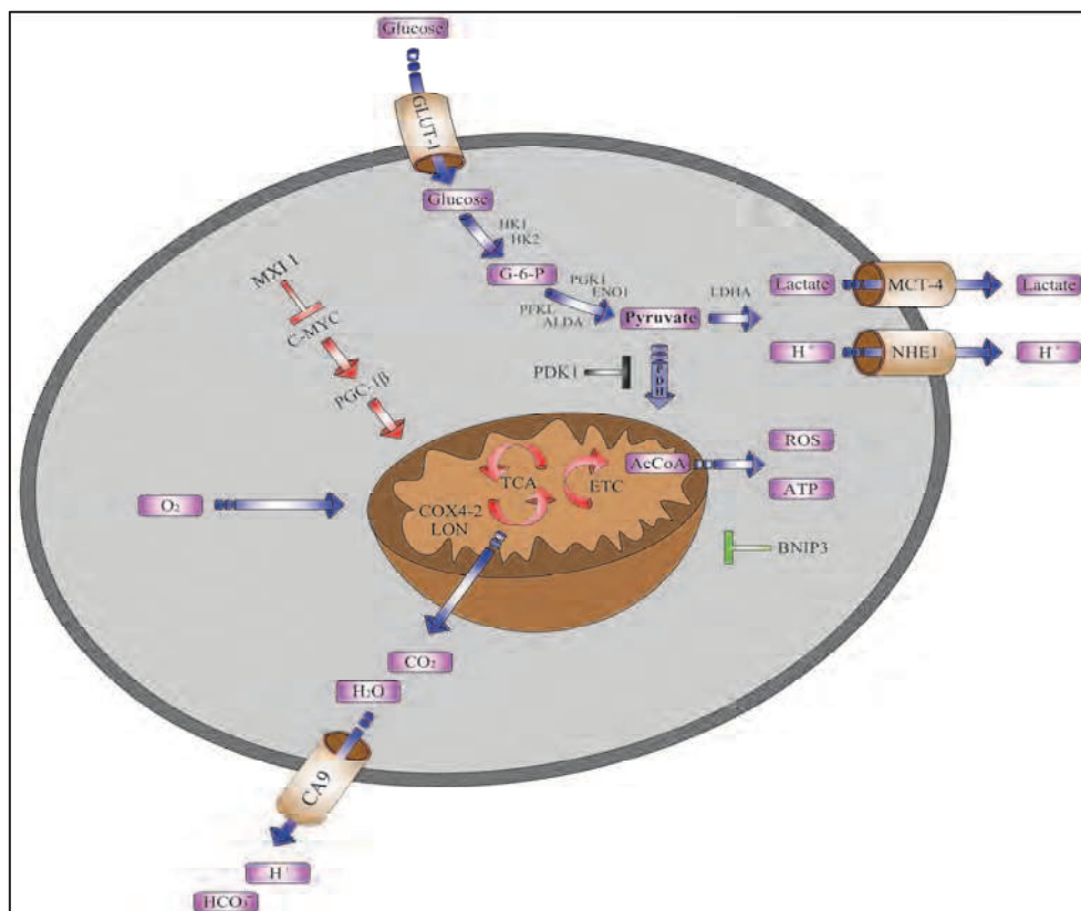
Fig. 5. Regulation of proteins required for glucose uptake and energy metabolism by HIF-1. Metabolic substrates and products are shown in purple and HIF-1-regulated gene products are shown in brown. Red arrows, mitochondrial biogenesis mediated by C-MYC (in renal carcinoma cells). Green blocked arrow, mitochondrial autophagy mediated by BNIP3 (in mouse embryo fibroblasts). AcCoA, acetyl coenzyme A; ALD, aldolase; CA9, carbonic anhydrase; COX, cytochrome c oxidase; ENO, enolase; G-6-P, glucose-6-phosphate; GLUT, glucose transporter; HK, hexokinase; LDH, lactate dehydrogenase; MCT, monocarboxylate transporter; NHE, sodium-hydrogen exchanger; PDH, pyruvate dehydrogenase; PDK, PDH kinase; PFK, phosphofructokinase; PGC, PPAR- \gamma co-activator; PGK, phosphoglycerate kinase.
