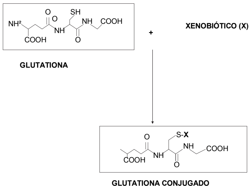
Fig. 1. Conjugation of glutathione to a generic xenobiotic (X) via catalysis by GSTs to form a conjugate of GST.
