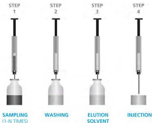
Fig. 5. MEPS procedure steps (SGE, 2009).
