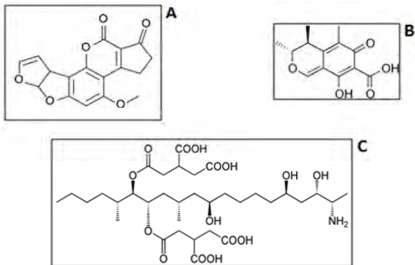
Fig. 1. Chemical structures of some common mycotoxins: aflatoxin B 1 (A), citrinin (B) and fumonisin B 1 (C).
