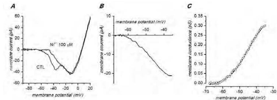
Fig. 8. Properties of the LVA calcium current. A - Voltage-clamp ramps were performed from -80 to +40 mV at a speed of 7 V/s in the presence of TTX ( 1 \mu\text{M} ), and after substitution of \text{Sr}^{2+} for \text{Ca}^{2+} ; the traces were corrected for leakage. Under these conditions, a distinct bump can be seen preceding the HVA calcium current (here peaking at -10 mV), which is selectively suppressed by \text{Ni}^{2+} 100 \mu\text{M} . B - Transient Ca-current generated using the protocol described in A calculated by subtracting the current-voltage curves in control and in the presence of 100 \mu\text{M} \text{Ni}^{2+} . The low- \text{Ni}^{2+} sensitive current (average from three cells) is activated at membrane potentials more positive than -60 mV. C - Conductance-voltage relationship of the low- \text{Ni}^{2+} sensitive current. The continuous line is a Boltzmann fit, with a midpoint at -45.3 mV and a maximum conductance of 0.35 nS. All recordings in this figure were performed from spontaneously bursting dissociated TH-GFP cells.
