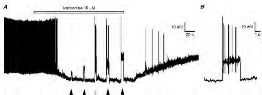
Fig. 11. Effect of blockers of h-channels on spontaneous firing. A - Ivabradine ( 10\ \mu\text{M} , bar) block of spontaneous activity; note the large hyperpolarization. At the times indicated by arrowheads, depolarising currents of increasing amplitudes were delivered. B - Enlargement of the response to the third injection of depolarising current (grey arrowhead) to show that the block of the h-current does not impair the spontaneous activity, provided that the membrane is brought back to resting values.
