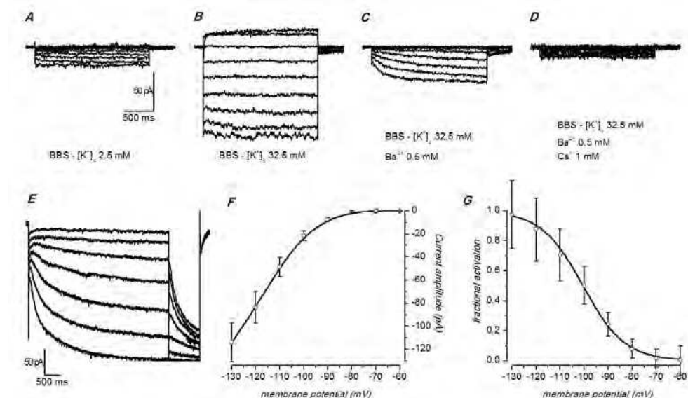
Fig. 9. Properties of the h-current. A,B - Currents activated by hyperpolarizing steps in normal saline and in high K + , respectively. C - Currents activated by hyperpolarization in high K + and after blockage of the K IR component with Ba 2+ 0.5 mM. D - Same as C after addition of a blocker of the h-current (Cs + 1 mM) E - Representative current traces for the analysis of activation. The membrane was held at -40 mV, depolarised to test voltages from -60 to -130 mV in 10 mV increments. I h tails were elicited in response to a second pulse to -130 mV, following test voltages (see methods for explanation) F - I/V relationship of the h-current for a group of 15 cells. G - Fractional activation of the h-current as a function of voltage.
