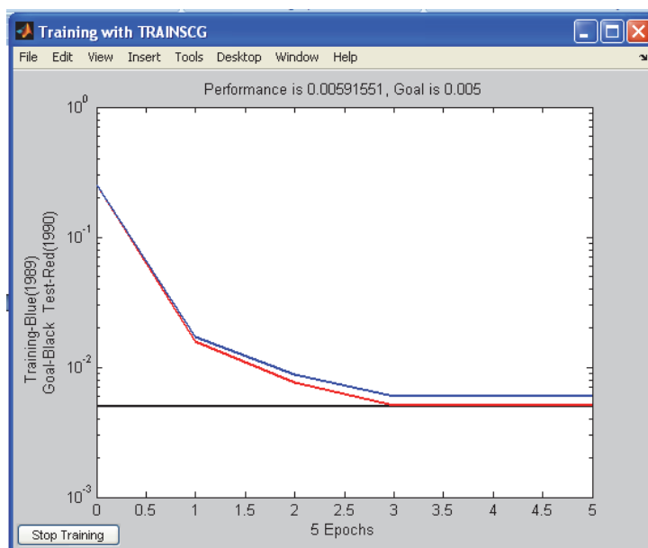
Fig. 5. Result of training ANN with Rainfall data of year 1989 and testing with Rainfall data of year 1990 using learning function trainscg
