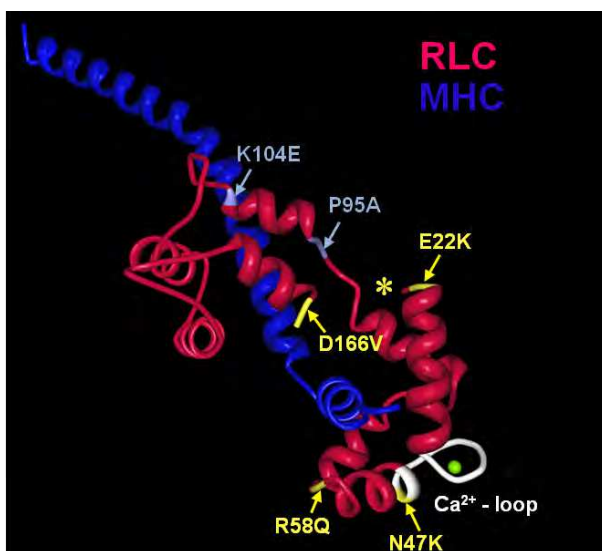
Fig. 3. Structure of the regulatory domain of scallop myosin (1WDC) (Houdusse & Cohen, 1996): Indicated are the FHC mutations, Ca 2+ -Mg 2+ binding site and the phosphorylation site. The MHC (myosin heavy chain) is labeled in dark blue, and the RLC (regulatory light chain) in red. Asterisks (*) depict the predicted location of A13T and F18L mutations and Ser-15 phosphorylation site (the region of RLC which is not resolved in all available vertebrate myosin crystal structures).
