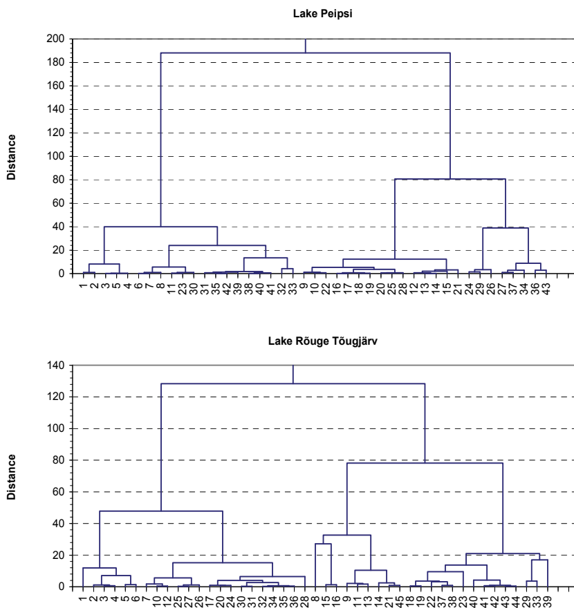
Fig. 7. Cluster analysis of Lake Peipsi and Lake Rõuge Tõugjärv sediment core samples from different depths (numbers indicate sediment depth in centimetres).
