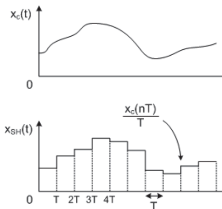
Fig. 2. Discrete-time signal x_c(t) processing for System I.
