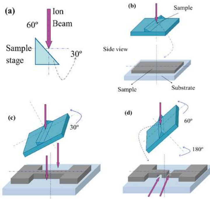
Fig. 3. FIB 3-D fabrication process (a) Scheme of the inclined plane has an angle of 60° with ion beam (where we mount sample). (b) The initial orientation of sample and sample stage. (c) Sample stage tilted by 30° anticlockwise with respect to ion beam and milling along ab -plane. (d) The sample stage rotated by an angle of 180° and also tilted by 60° anticlockwise with respect to ion beam and milled along the c -axis.
