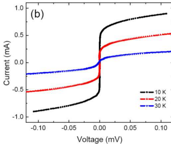
Fig. 11. I-V characteristics of the device without microwave irradiation at different temperature of 10, 20, and 30 K. The critical current density J_c about 2.2 \times 10^5 \text{ A/cm}^2 is measured at 20 K.
