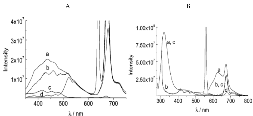
Fig. 2. A. Emission spectra of olive oil with \lambda_{ex} = 320 nm. (a) front face spectrum; (b) right angle spectrum with the absorption correction; (c) absorption spectrum of the oil multiplied by 10^6 ; (d) right angle spectrum without the absorption correction. B. Emission spectra of olive oil with \lambda_{ex} = 280 nm. (a) front face spectrum; (b) right angle spectrum with the absorption correction and multiplied by 3.7; (c) front face spectrum, second-order corrected; (d) right angle spectrum. Reprinted with permission from Zandomeneghi et al. 2005. Copyright 2005 American Chemical Society.
