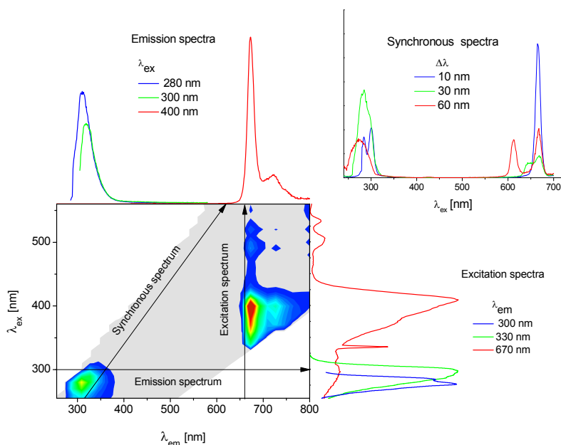
Fig. 1. Different types of fluorescence spectra; fluorescence spectra of a diluted sample of extra virgin olive oil (1%, v/v, in n-hexane) are shown as an example.
