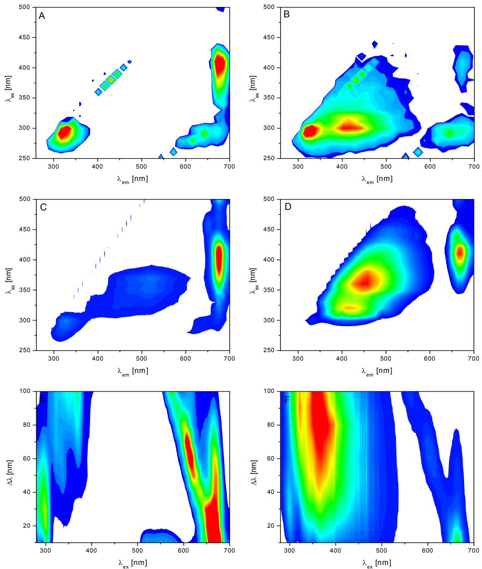
Fig. 3. Fluorescence spectra of extra virgin and refined olive oil: A. Total fluorescence spectrum of diluted olive oil, 1% in n-hexane, B. Total fluorescence spectrum of diluted refined olive oil, 1% in n-hexane, C. Total fluorescence spectrum of undiluted extra virgin olive oil, front face geometry, D. Total fluorescence spectrum of undiluted refined olive oil, front face geometry, E. Total synchronous fluorescence spectrum of undiluted extra virgin olive oil, front face geometry, F. Total synchronous fluorescence spectrum of undiluted refined olive oil, front face geometry (Sikorska et al., 2011).
