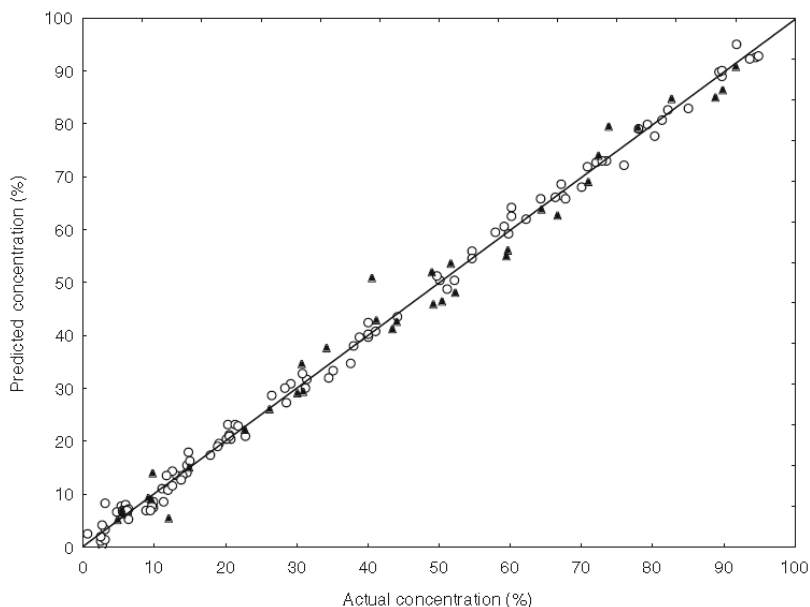
Fig. 6. Predicted versus actual concentrations of sunflower oil in virgin olive oil at a wavelength interval of 80 nm: open circles - calibration samples, filled triangles - validation samples. Reprinted with permission from Poulli et al., 2006. Copyright 2006, Springer.
