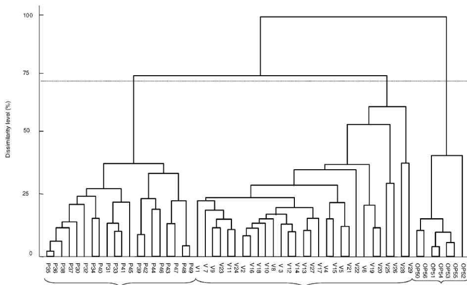
Fig. 5. Dendrogram of the 56 x 861 unfolded matrix ( \lambda_{ex}=300-400 nm, \lambda_{em}=400-600 nm) using the Euclidean distance as similarity measure and the average linkage method. The distance is expressed as a percentage of dissimilarity (normalized and autoscaled spectra): virgin V, pure, P; and olive-pomace, OP oils. Reprinted with permission from Guimet et al., 2004a. Copyright 2004, American Chemical Society.
