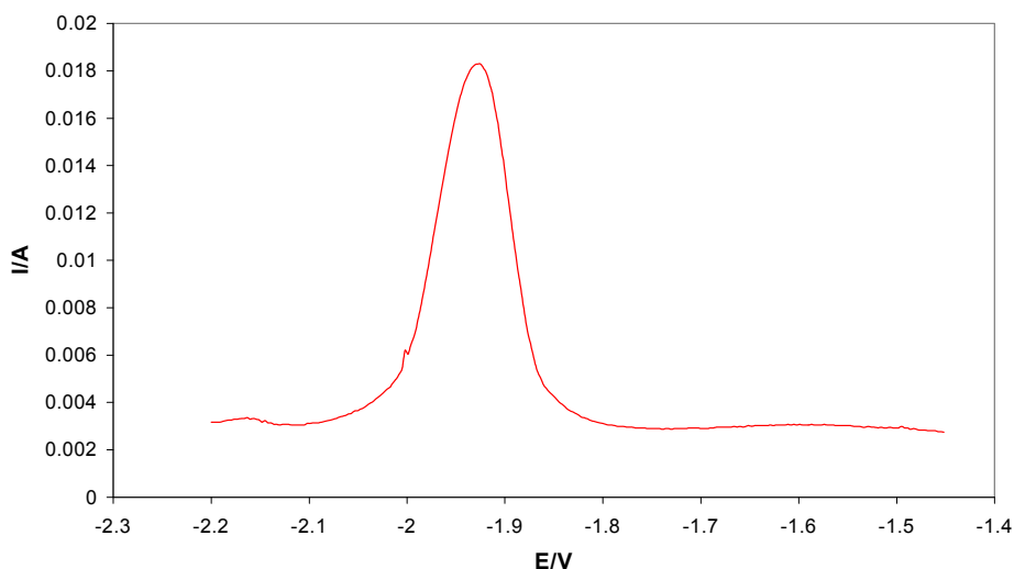
Fig. 9. Differential pulse voltammogram of \text{NaCl}\cdot 2\text{CsCl}\cdot \text{CmCl}_3 melt at 923 K. [\text{Cm(III)}] = 4.4 \cdot 10^{-2} \text{ mol}\cdot\text{kg}^{-1}
