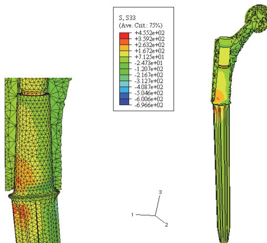
Fig. 3. S33 stress distribution (MPa)
