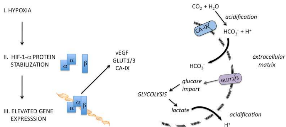
Fig. 2. Regulation of extracellular acidification and glycolysis in hypoxic cells. The transcription factor HIF-1 \alpha is degraded in normoxic cells through the VHL tumour suppressor protein. In response to lowered oxygen concentrations, HIF-1 \alpha is stabilized and forms a complex with HIF-1 \beta to induce adaptive gene products. Some of these gene products include CA-IX and GLUT1/3 that coordinately mediate glycolysis and acidification that together drive survival in cancer cells. GLUT1/3 drives glucose transport where cellular energy is derived from glycolysis. CA-IX catalyzes extracellularly condensation of carbon dioxide and water to hydrogen ions and carbonate. Carbonate ions are transported intracellularly where CA-II neutralizes hydrogen ions and carbonate to carbon dioxide, which is transported from the cell.
