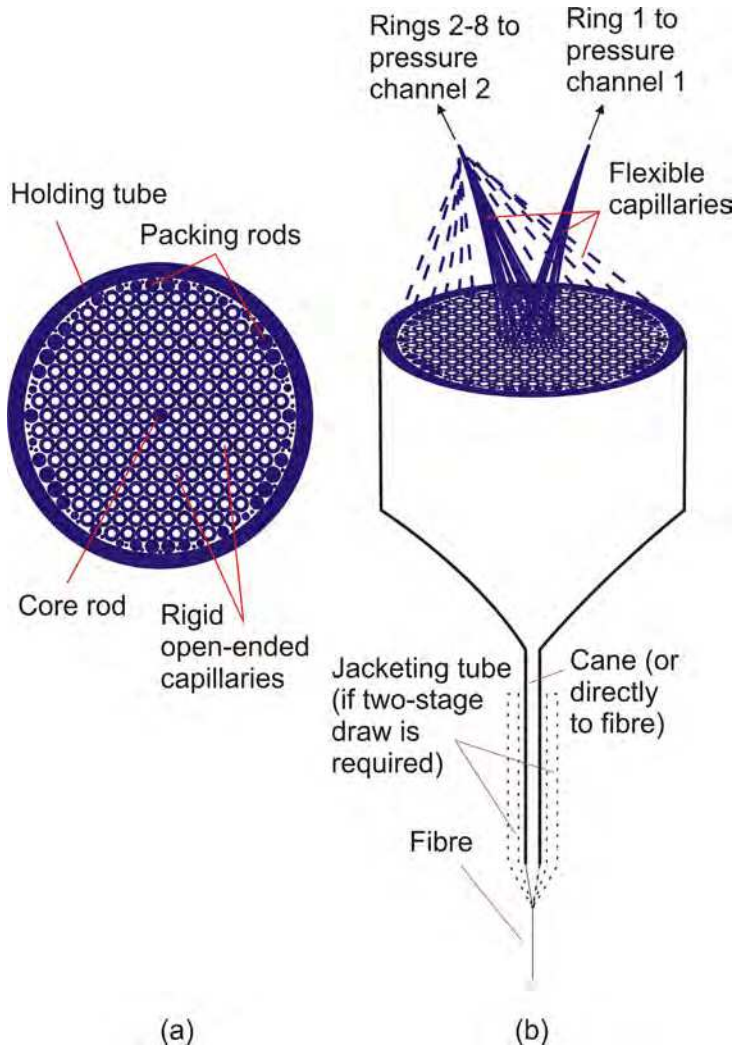
Fig. 7. A schematic of the proposed MOF taper fabrication method. (a) End-view of the stacking arrangement. (b) Shows the inserted flexible capillaries extension which can be connected to different pressure regulatory channels.
