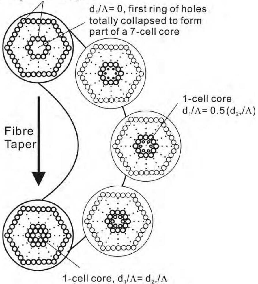
Fig. 1. A schematic of the proposed MOF taper scheme. Rings 2-8 consisted of large air-holes. The core-size is reduced by introducing the innermost ring of holes (ring 1). A 7-cell defect solid-core is found in the beginning of the fibre , which is formed partly by totally collapsing the holes in ring 1. A single-cell defect solid-core is found at the end of the fibre.
