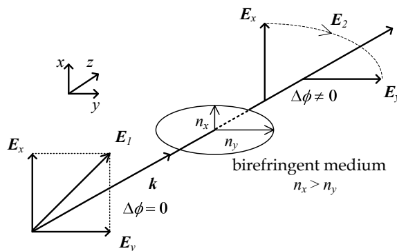
Fig. 5. State of polarization change in birefringent medium.
