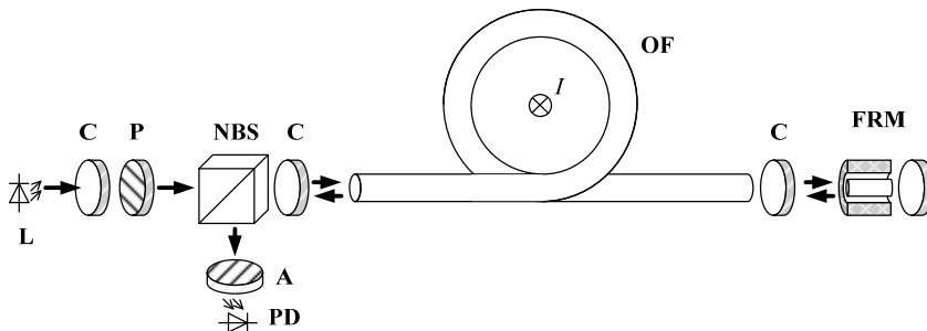
Fig. 16. Fiber optic polarimetric current sensor utilizing Faraday rotation mirror.
