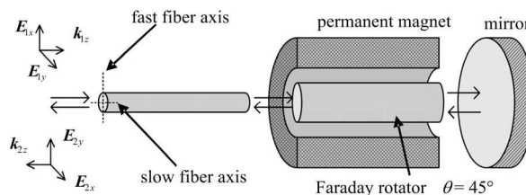
Fig. 15. Principle of Faraday rotation mirror.
