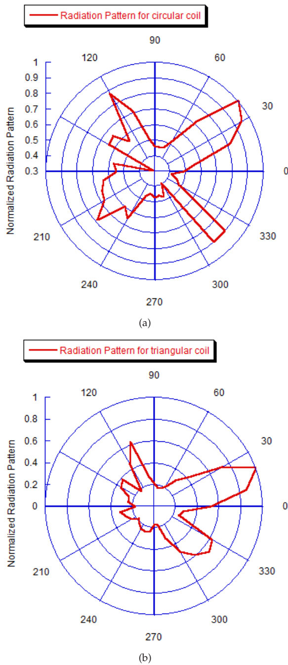
Fig. 10. Radiation pattern for (a) circular and (b) triangular coils.
