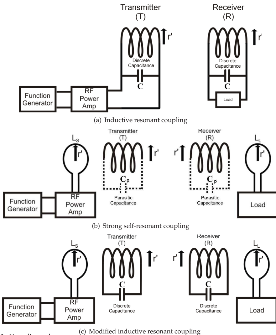
Fig. 1. Coupling schemes
