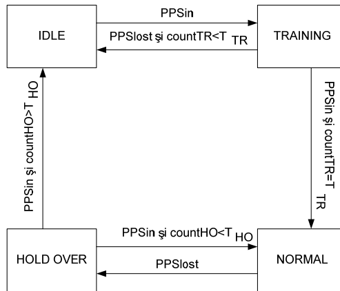
Fig. 3.6 FSM for synchronization block
