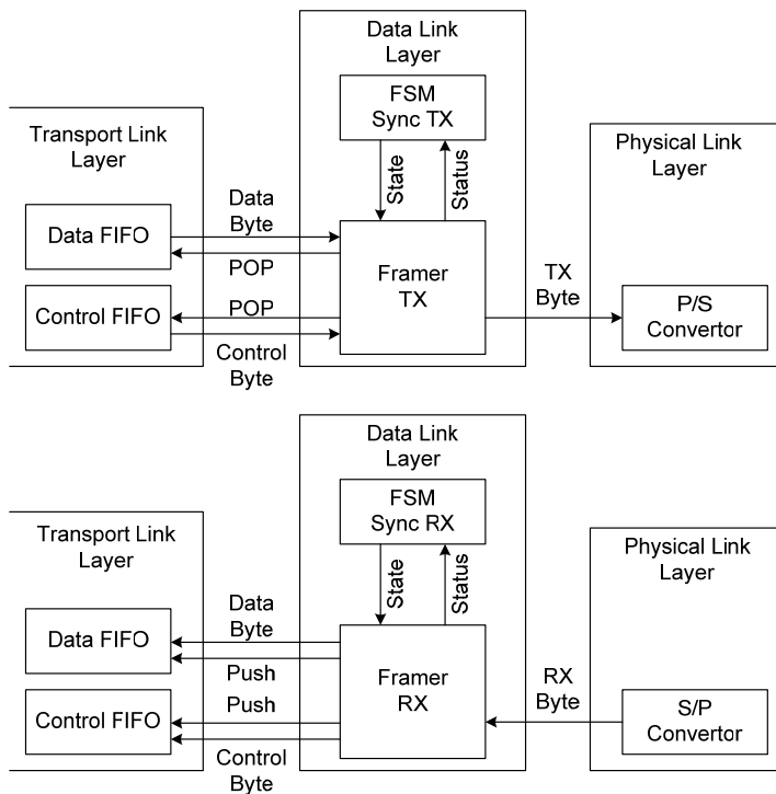
Fig. 4.7 Interface Tx and Rx chains
