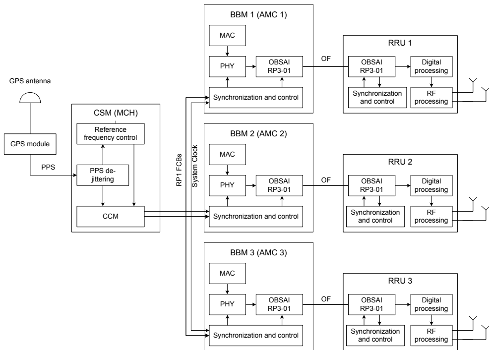
Fig. 2.4 WiMAX BS for a cell with 3 sectors
