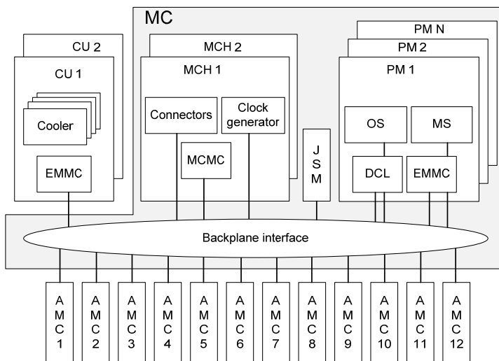
Fig. 2.1 MicroTCA – Block scheme
