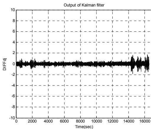
Fig. 3.11 DIFFdj values in clock periods
