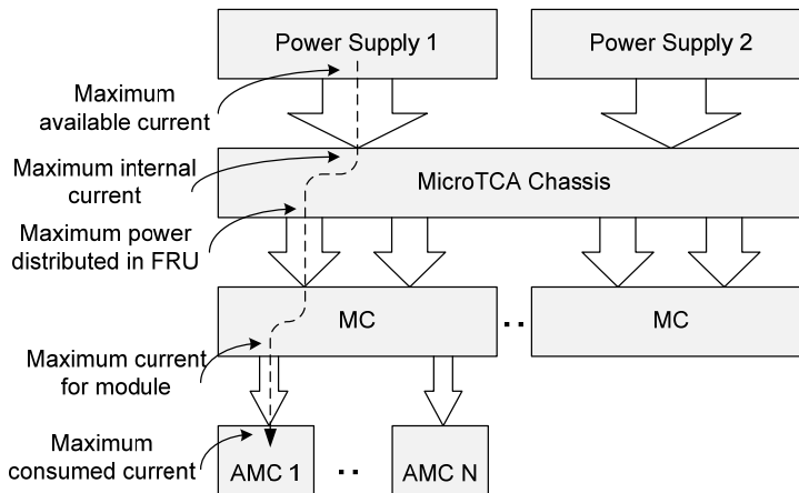
Fig. 2.2 Power distribution infrastructure
