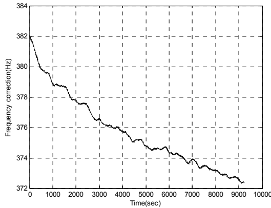
Fig. 3.8 Mean of frequency deviation
