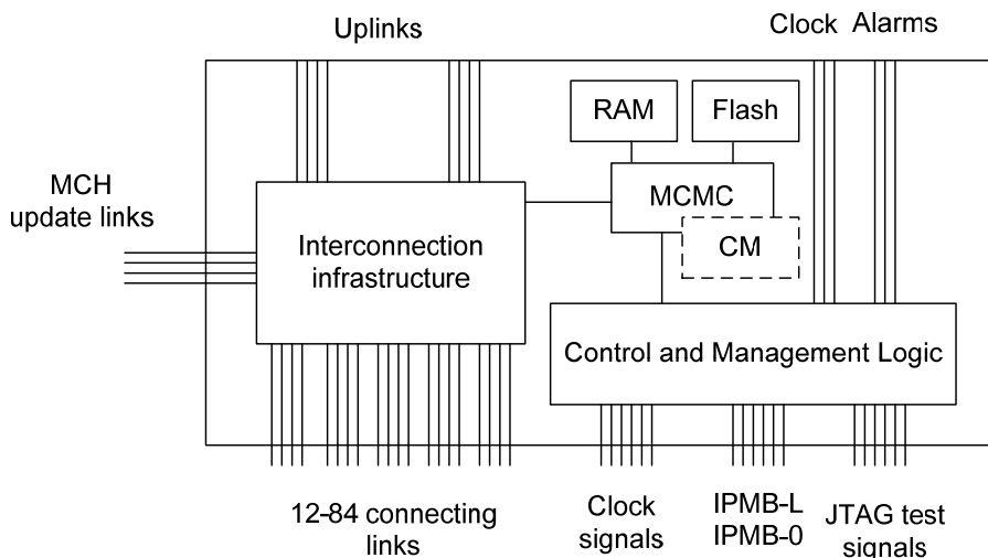
Fig. 2.3 MCH - Block scheme
