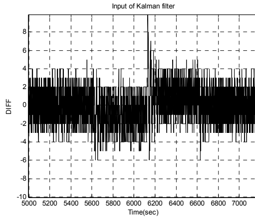
Fig. 3.12 DIFF values in clock periods
