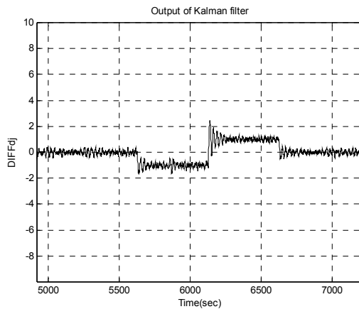
Fig. 3.13 DIFFdj values in clock periods
