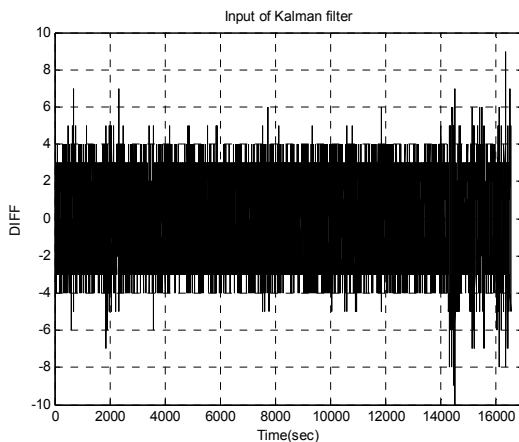
Fig. 3.10 DIFF values in clock periods
