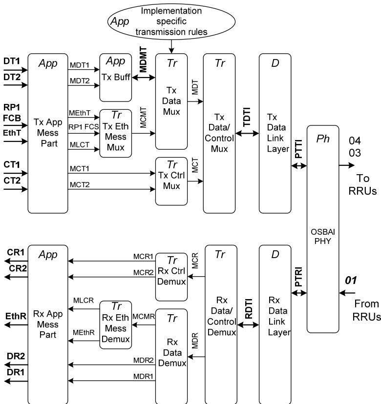
Fig. 4.5 Block scheme for BBM RP3-01 interface
