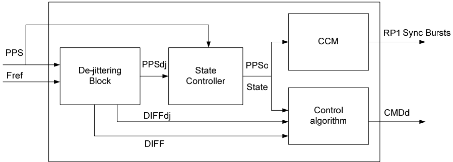
Fig. 3.2 The bloc scheme of the digital part
