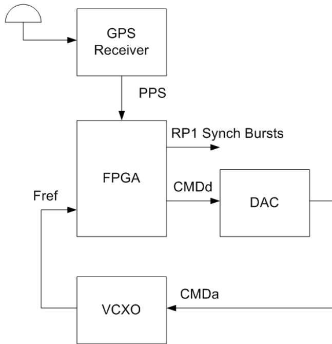
Fig. 3.1 Controlling scheme
