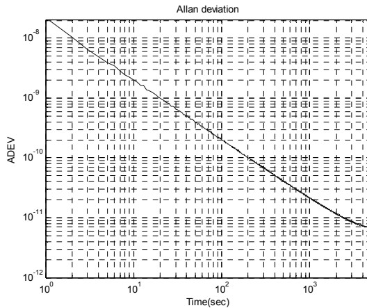
Fig. 3.5 PPS jitter Allan deviation
