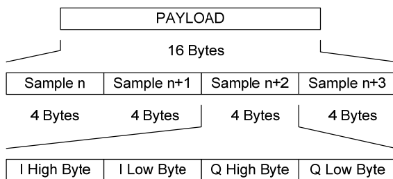
Fig. 4.2 802.16 payload mapping
