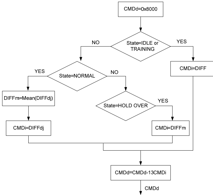
Fig. 3.7 Control Algorithm
