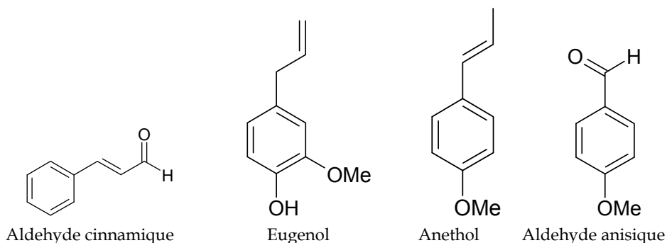
Fig. 4. Examples of aromatic compounds.
