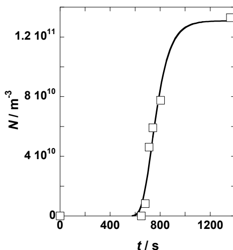
Fig. 3. Time course of the number of observed microcrystals at T = 20 °C, C = 27.07 mgmL -1 , and P = 100 MPa (Maruoka et al., 2010). Solid curve indicates a Gompertz function.
