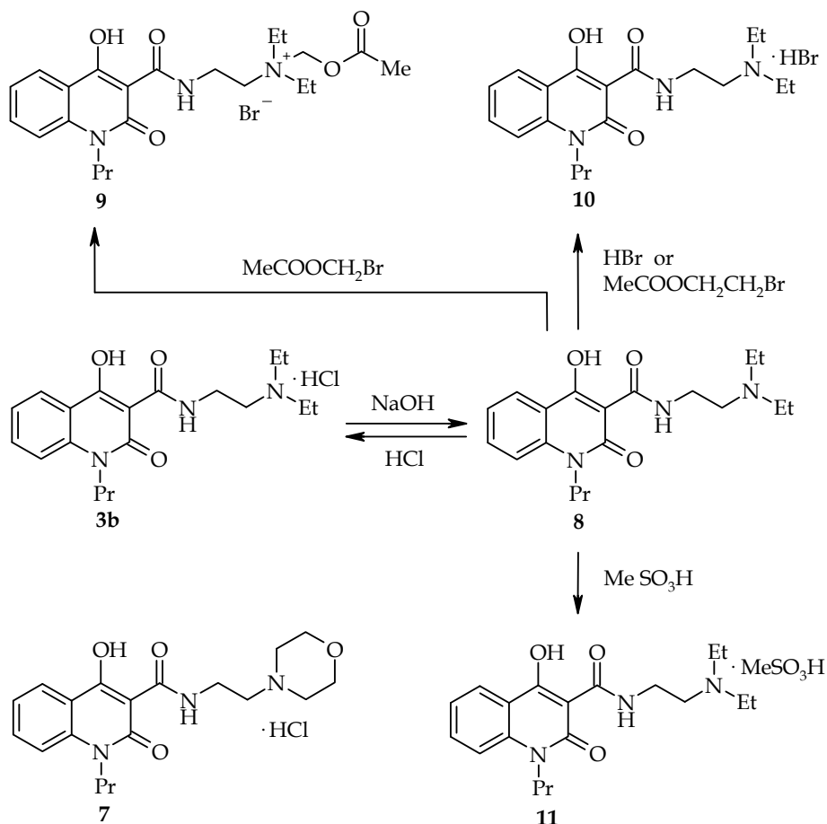
Fig. 3. Modification of Chinoxicaïne into pro-drugs
