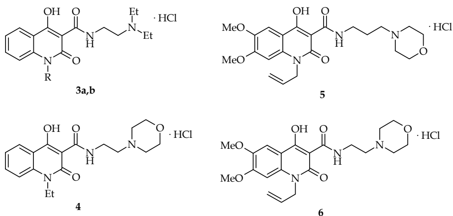
Fig. 2. Biologically active 4-hydroxy-2-oxo-1,2-dihydroquinoline-3-carboxamides
