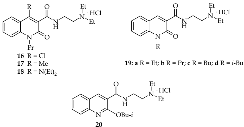
Fig. 8. Modification of 4-OH-group of Chinoxicaine
