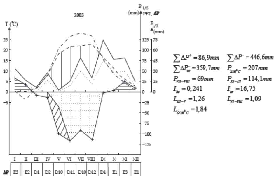
Fig. 6. Climate charts for years 2002 and 2003 and characteristics sizes determined for reviewed site
