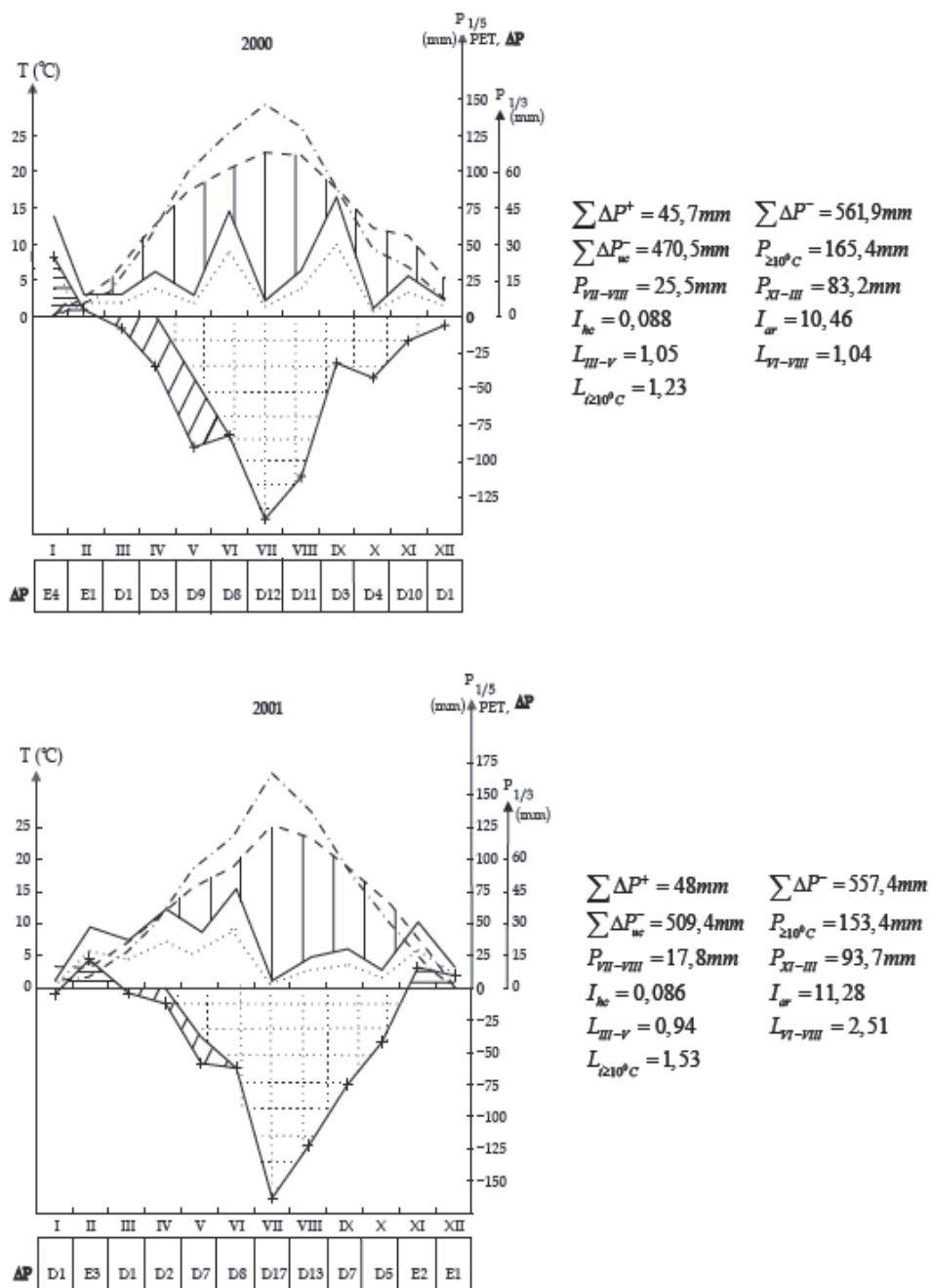
Fig. 5. Climate charts for years 2000 and 2001 and characteristics sizes determined for reviewed site
