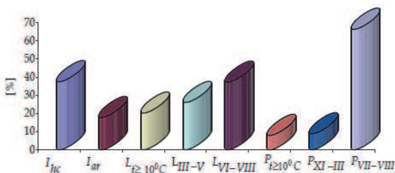
Fig. 10. Increases of the average annual percentage values of main indices for the period 2000 - 2009 for the studied site comparing to the specific values of the reference period 1961 - 1990.
