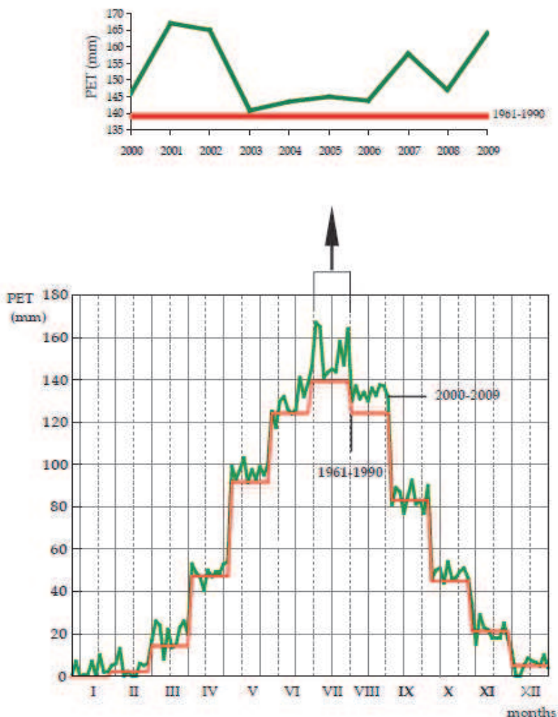
Fig. 12. Interannual distribution of PET in the period 2000 - 2009 comparing to the annual average of the reference period 1961 - 1990 for the studied area.
