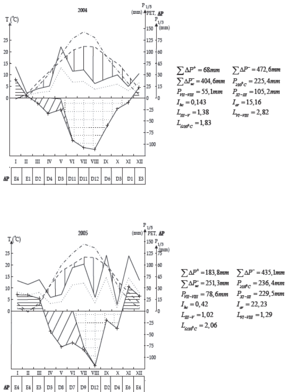
Fig. 7. Climate charts for years 2004 and 2005 and characteristic sizes determined for reviewed site
