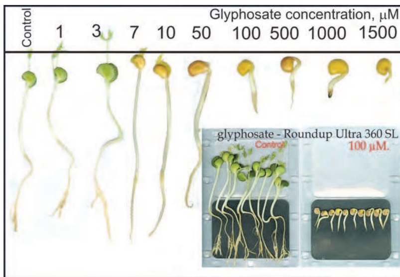
Fig. 7. PHYTOTOKKIT is used to determine phytotoxicity of soil contaminated different glyphosate concentration.
