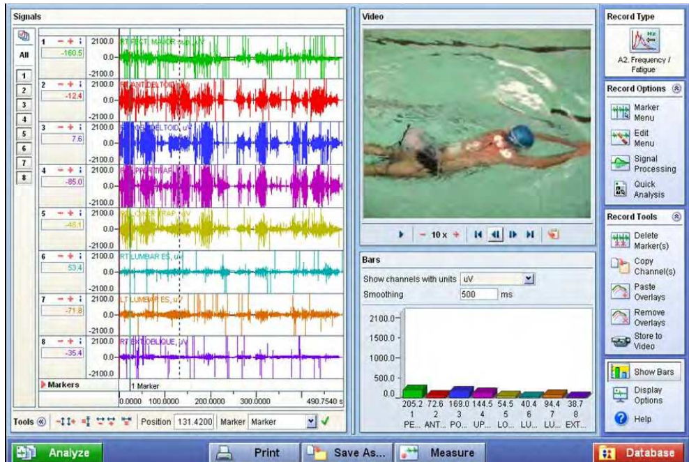
Fig. 6. WaS-EMG: Recording of swimming (Pánek et al, 2010).
