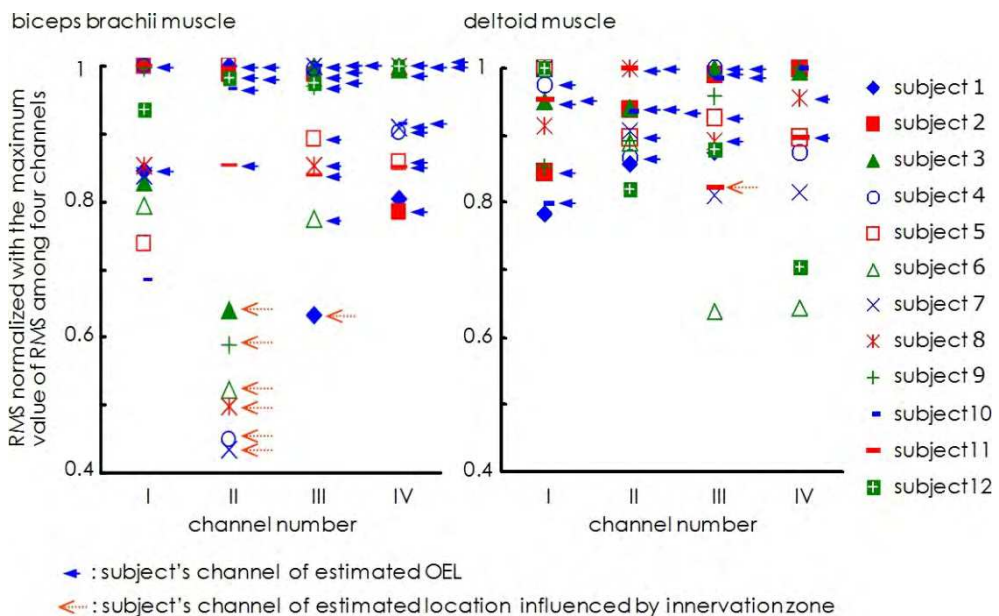
Fig. 12. RMSs of raw EMG signals for the subject channels depicted in Fig. 11.
