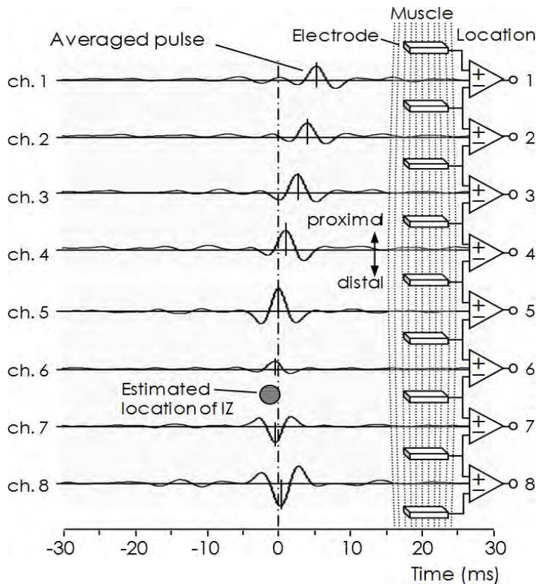
Fig. 7. Example of the generation of averaged pulses.
