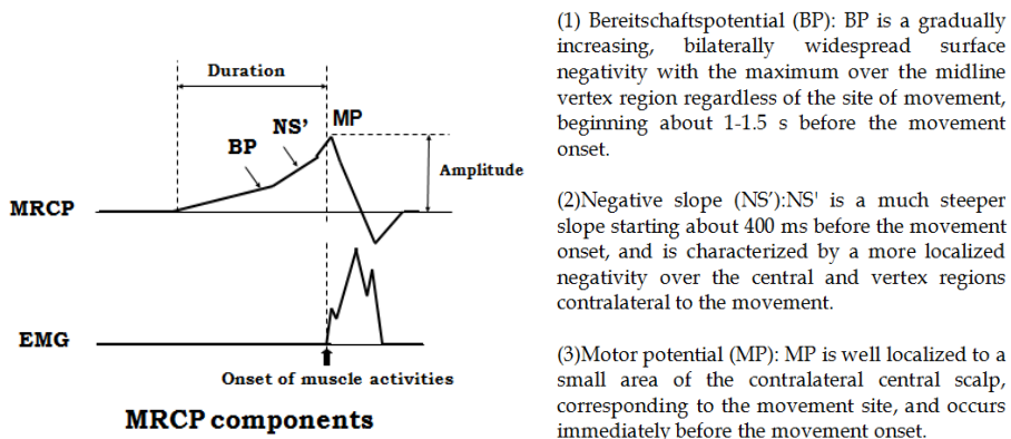
Fig. 4. Schema of MRCP waveform.
