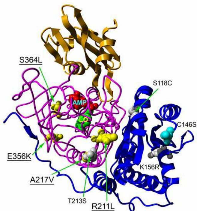
Fig. 10. Homology model of L. mingrelica luciferase showing the location of substitutions in the mutant 4TS. Four key thermostabilizing mutations are underlined. LO is AMP – luciferyl and adenylate groups of DLSA (5'-O-[N-(dehydroluciferyl)-sulfamoyl] adenosine). Subdomains A, B and C are depicted in blue, magenta and orange, respectively
