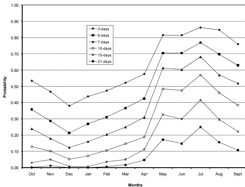
Fig. 1. Probability of a dry spell lasting \geq n days in each month estimated using the raw data from 1983-2005 at the semi-arid ecotope. ( n=3, 5, 7, 15, 21 ).
