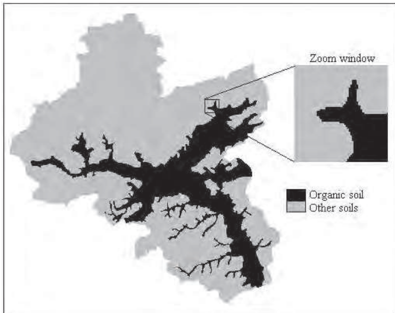
Fig. 7. Organic soil map with Boolean boundaries
