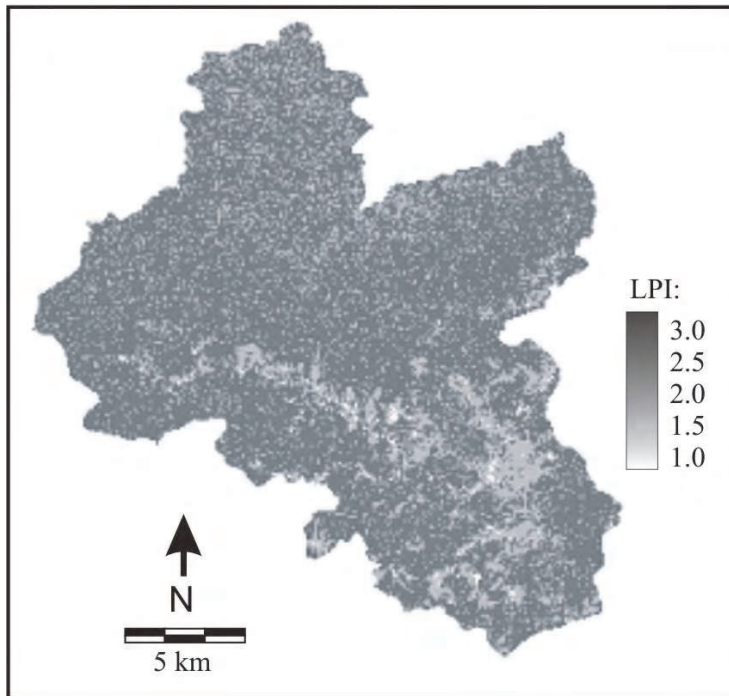
Fig. 2. Leaf Pigment Index (LPI) map
