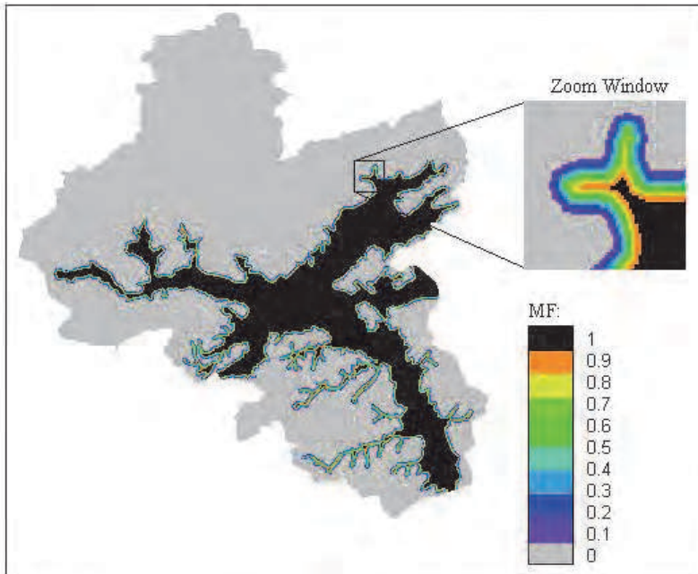
Fig. 6. Organic soil map with fuzzy boundaries
