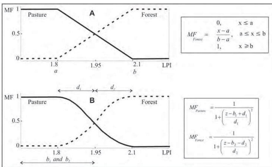
Fig. 4. Membership functions: (A) linear; (B) bell-shaped
