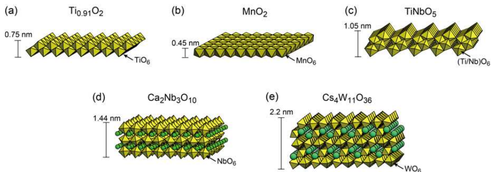
Fig. 2. Structures of selected oxide nanosheets. (a) \text{Ti}_{0.91}\text{O}_2 , (b) \text{MnO}_2 , (c) \text{TiNbO}_5 , (d) \text{Ca}_2\text{Nb}_3\text{O}_{10} , (e) \text{Cs}_4\text{W}_{11}\text{O}_{36} .
