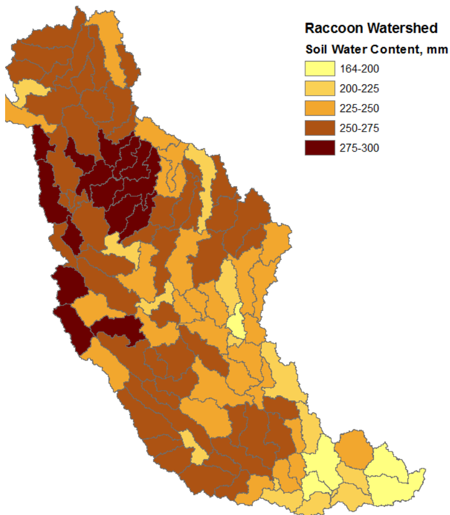
Fig. 8. Soil moisture content predicted by SWAT at subwatershed scale on a long-term basis
