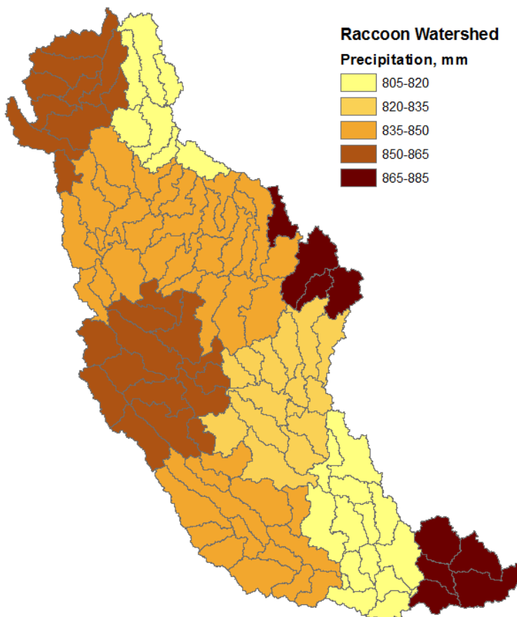
Fig. 5. Spatial representation of precipitation on a long-term annual basis
