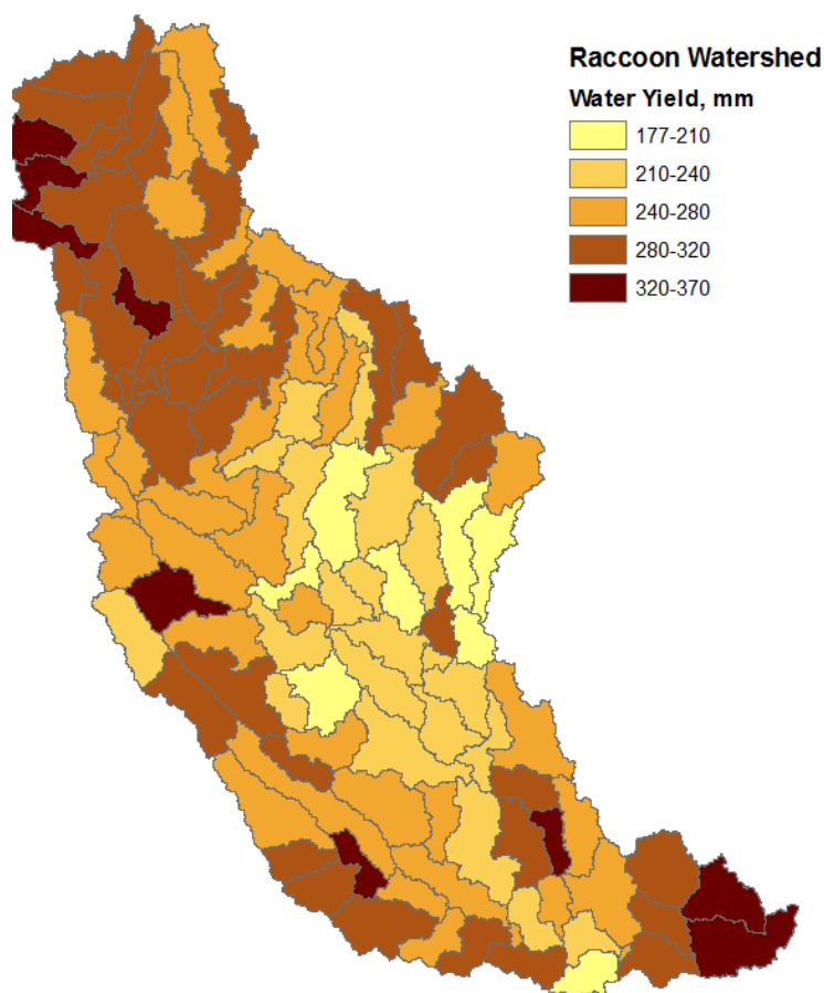
Fig. 7. Total water yield distribution as predicted by SWAT on a long-term basis
