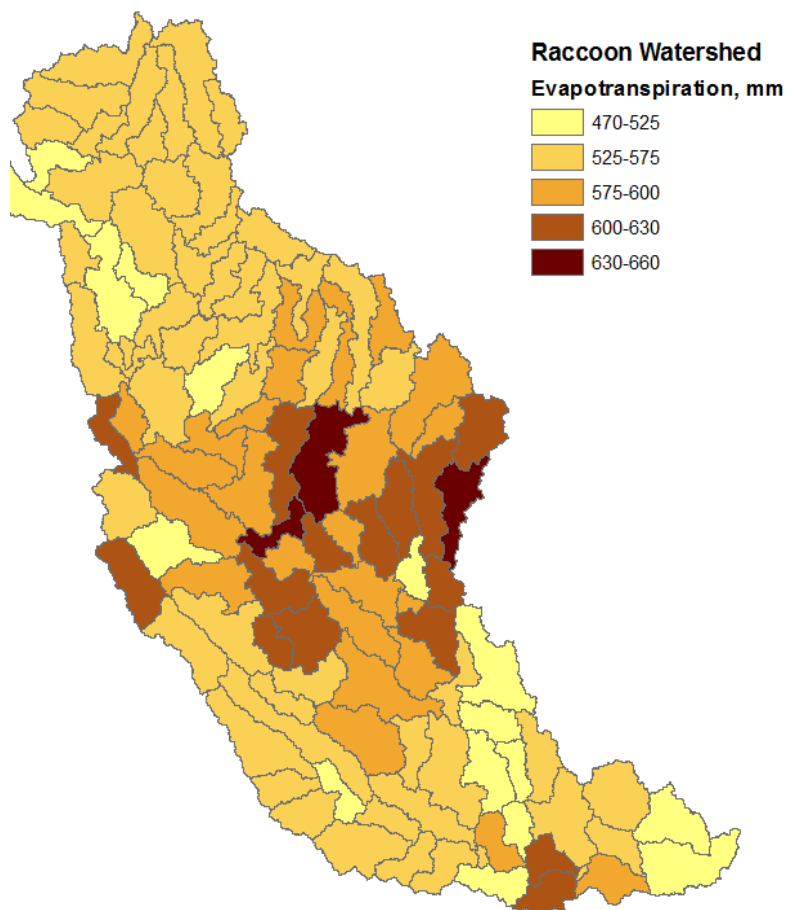
Fig. 6. Estimated evapotranspiration (ET) over a subwatershed scale on a long-term annual basis
