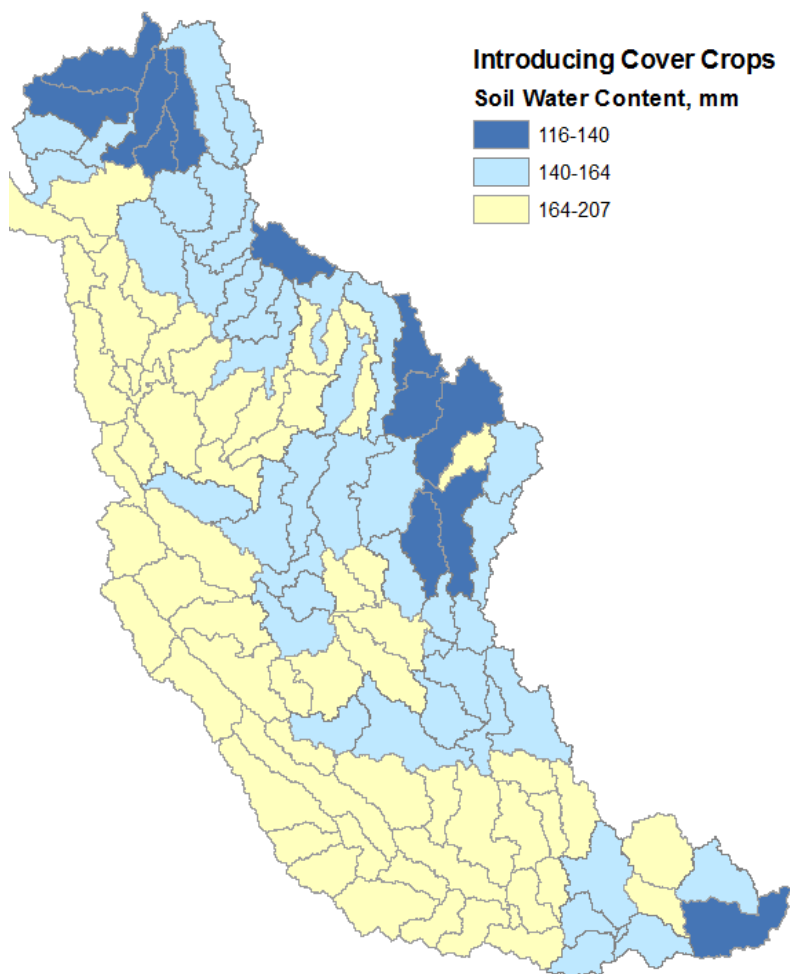
Fig. 9. Soil moisture content (after introducing winter cover crop) as predicted by SWAT at subwatershed scale on a long-term basis
