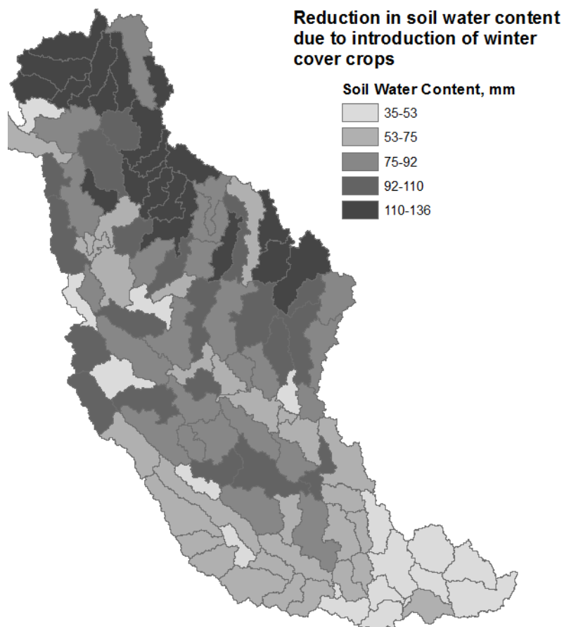
Fig. 10. Reduction in soil moisture content due to inclusion of winter cover crops in standard corn-soybean rotation on a long-term basis
