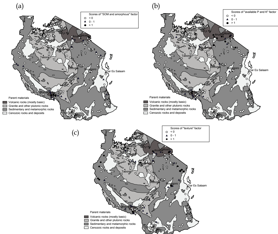
Fig. 3. Distribution patterns of scores of (a) "SOM and amorphous," (b) "available P and K," and (c) "texture" factors in relation to geological conditions
