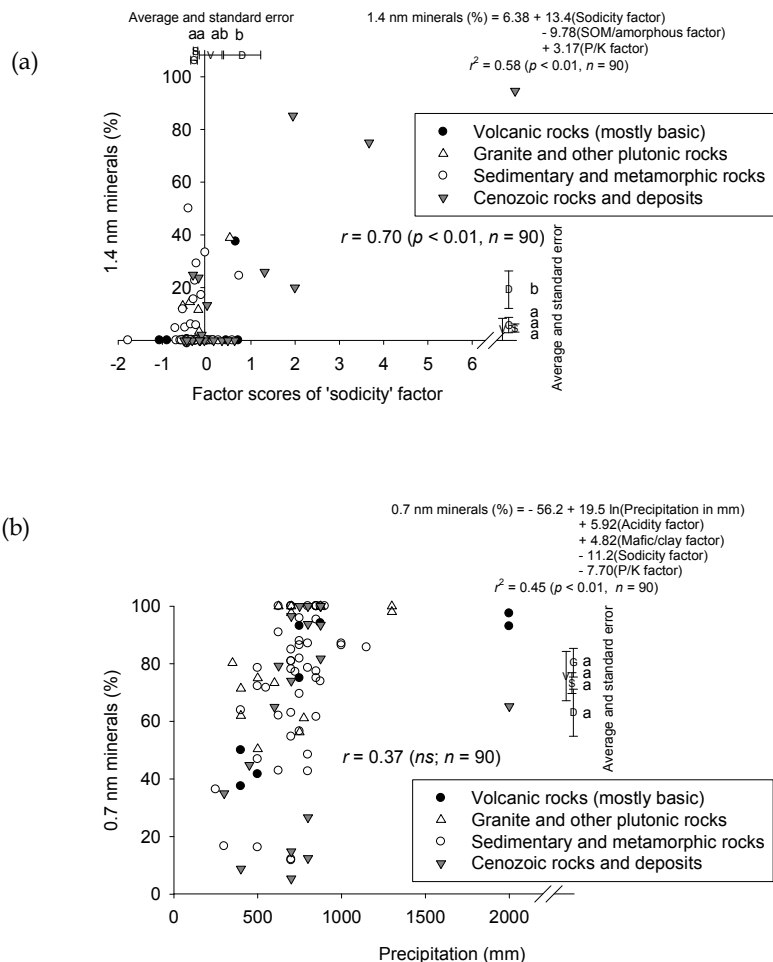
Fig. 6. Relationships between clay mineralogy and soil and climatic factors. Abundances of (a) 1.4 nm and (b) 0.7 nm minerals
