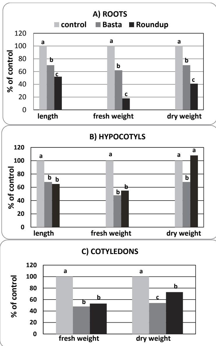
Fig. 1. The influence of Basta and Roundup on growth parameters of 7-day old cucumber seedlings. Values with the same letter above the bars do not differ significantly at P \leq 0.05 .
