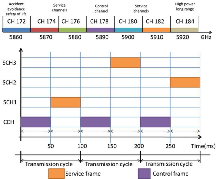
Fig. 1. Channels available for 802.11p
