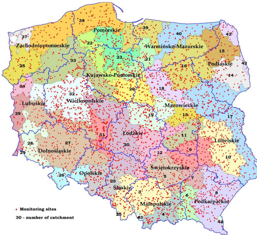
Fig. 1. Localization of the monitoring sites in Poland
