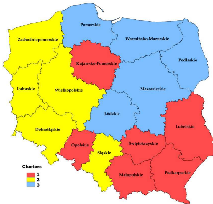
Fig. 2. Regional distribution of \text{NO}_3 - \text{N} losses over winter in Poland ( \text{kg N} \cdot \text{ha}^{-1} ) (see Table 12)
