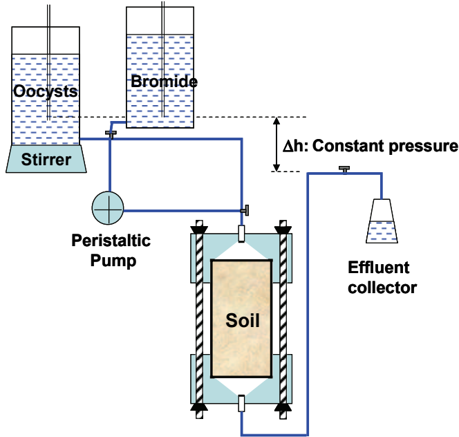
Fig. 2. A schematic diagram of the soil column experiment setup employed in the Br- and oocysts breakthrough study under a constant pressure (CP, Δh=22 cm in this study) or under a constant flux (CF) controlled by a peristaltic pump
