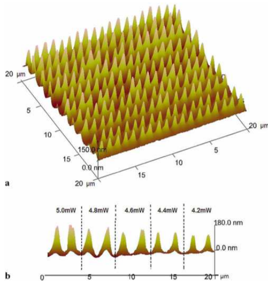
Fig. 14. AFM 3D photos of pattern structures in Fig. 3(a) kept the temperature at 100°C for 1 h. (a) The AFM 3D photos of pattern structures. (b) The lateral photos of the pattern structures in (a).
