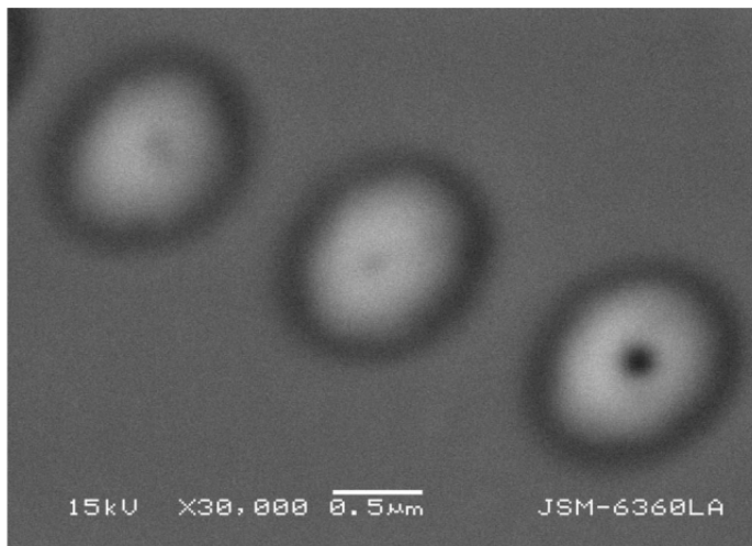
Fig. 4. SEM analysis for bumps formed at laser power of 3.85 , 3.90 and 4.0mW .
