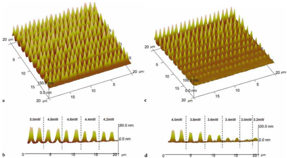
Fig. 11. Pattern structures written on multilayered ZnS-SiO 2 /AgOx/ZnS-SiO 2 films by green laser ( \lambda = 488 \text{ nm} ) in different laser processing parameters. (a) The AFM 3D photos of pattern structures written by higher laser power. (b) The lateral photos of the pattern structures in (a). (c) The AFM 3D photos of pattern structures written by lower laser power. (d) The lateral photos of the pattern structures in (c).
