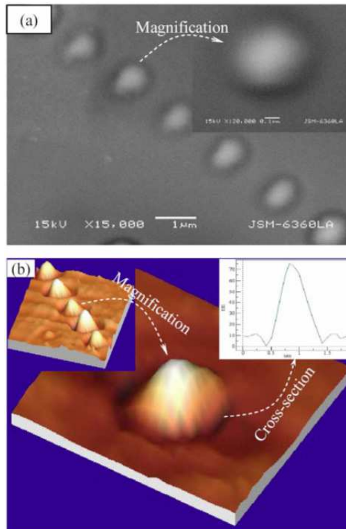
Fig. 3. Bumps formed at laser power 3.8mW : (a) SEM analysis and (b) AFM analysis.
