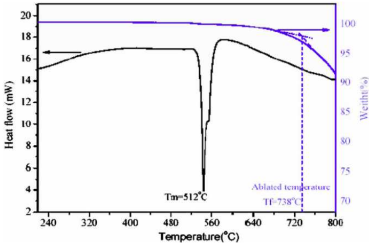
Fig. 6. DSC analysis for \text{Ag}_8\text{In}_{14}\text{Sb}_{55}\text{Te}_{23} thin films.
