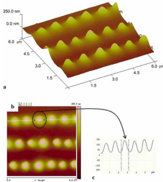
Fig. 13. Amplification photos of pattern structures chosen from Fig. 3(a). (a) The AFM 3D photos of pattern structure. (b) The chosen area of AFM analysis (marked by the line). (c) AFM analysis of the pattern structure in (b).
