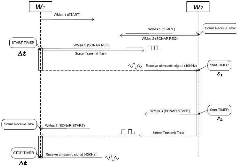
Fig. 10. Distance measurement with the CTOF method
