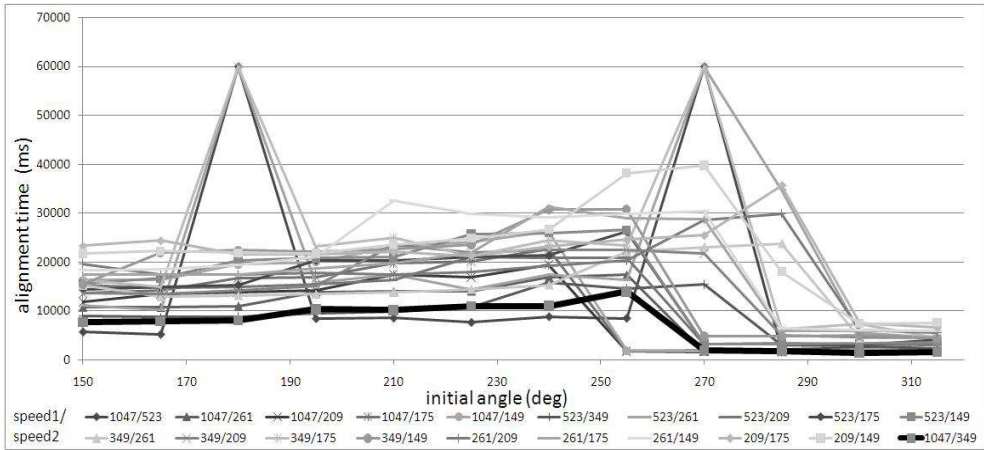
Fig. 9. Inter-robot alignment in the case of the transducers mounted on the turret
