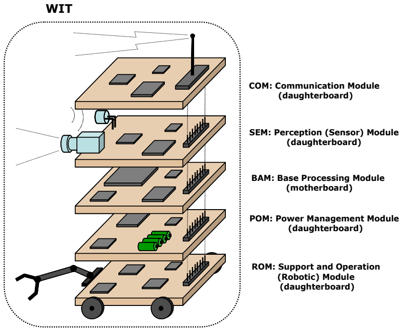
Fig. 2. Diagram of the Wireless Intelligent Terminal
