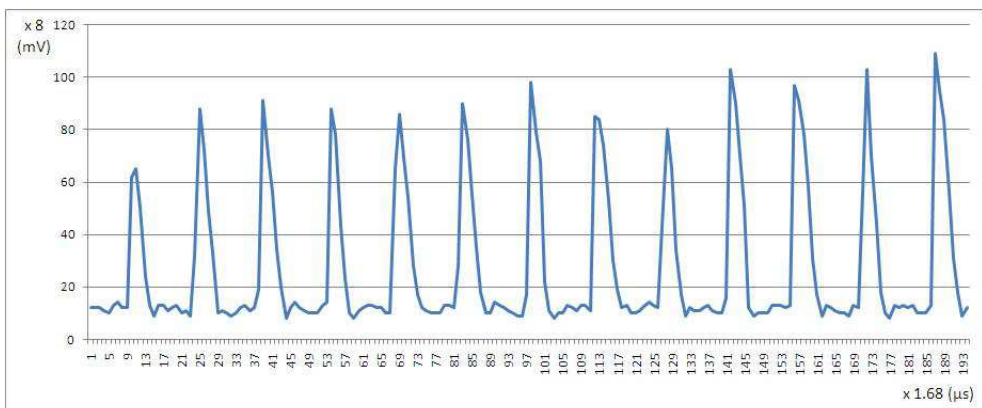
Fig. 11. Amplitude of the received ultrasonic signal, after amplification
