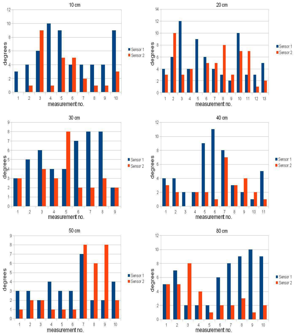
Fig. 14. Maximum variation of the correction angle for experimental alignment procedures
