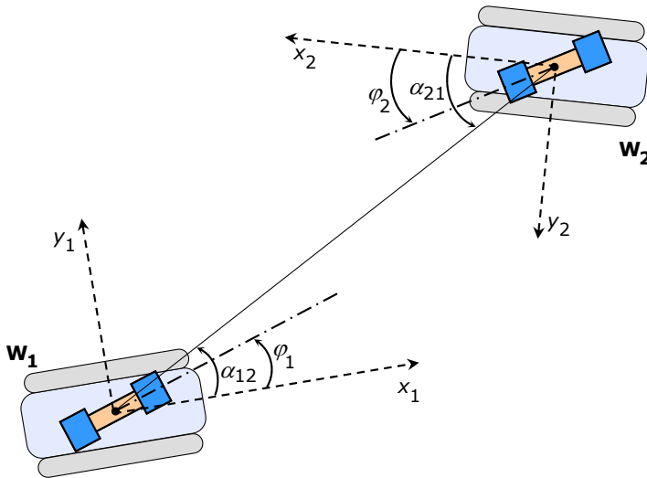
Fig. 5. Key angles on the alignment process
