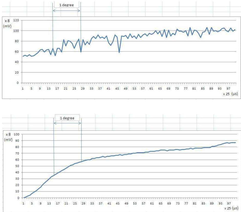
Fig. 12. Received signal without filtering (up) and after the Kalman filtering (down)
