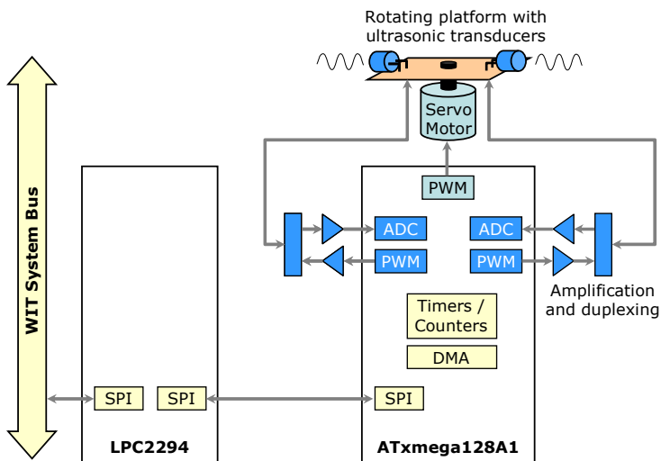
Fig. 3. Schematic of the WIT Perception Module
