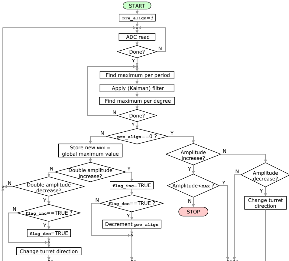
Fig. 6. Robotic alignment algorithm
