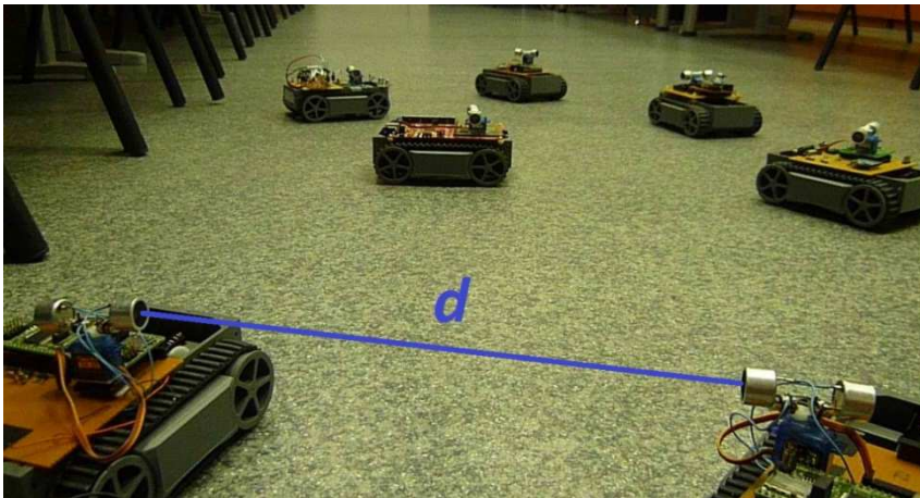
Fig. 4. Inter-robot alignment process
