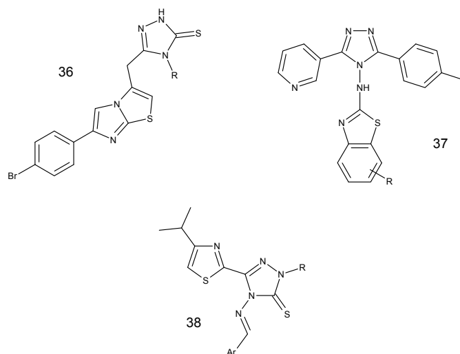
Fig. 10. Triazole derivatives as anti-TB agents.
