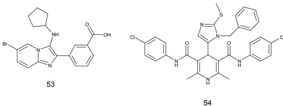
Fig. 17. Pyridine derivatives with potential activity anti-TB.
