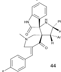
Fig. 13. Spiro-pyrrolothiazoles derivative with anti-TB activity.
