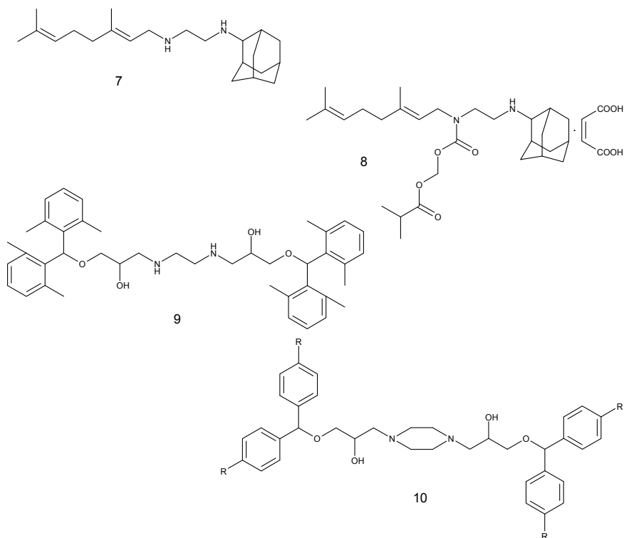
Fig. 2. Structure of SQ109 and analogs.
