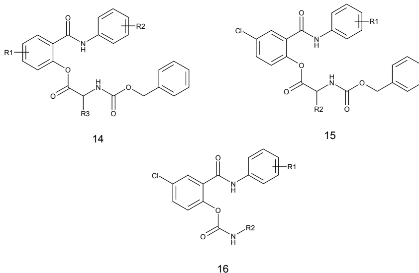
Fig. 4. General structure of salicylanilides derivatives with anti-TB activity.
