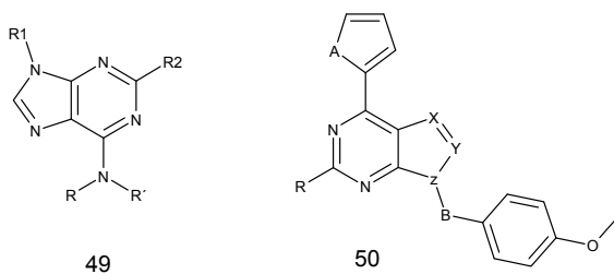
Fig. 15. Purine derivatives as anti-TB agents.
