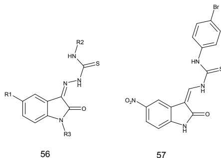
Fig. 19. General structure of 1 H -indole-2,3-dione 3-thiosemicarbazone with anti-TB activity.
