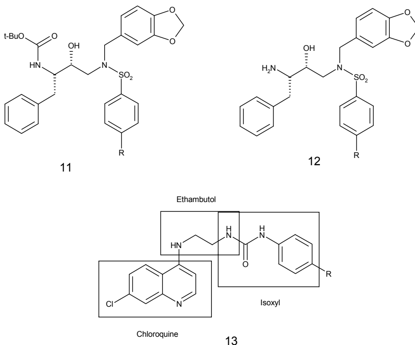
Fig. 3. Ethambutol analogs as anti-TB agents.
