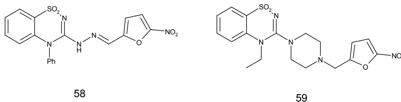
Fig. 20. Benzothiadiazine derivatives as anti-TB agents.
