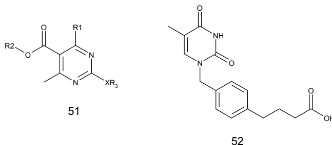
Fig. 16. General structure of pyrimidine derivatives as anti-TB agents.
