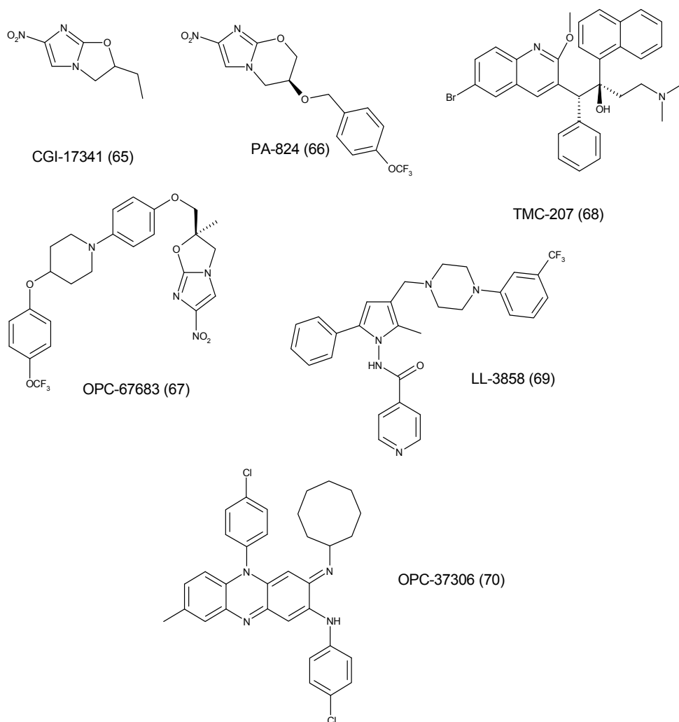
Fig. 24. Anti-TB compounds in clinical trials.
