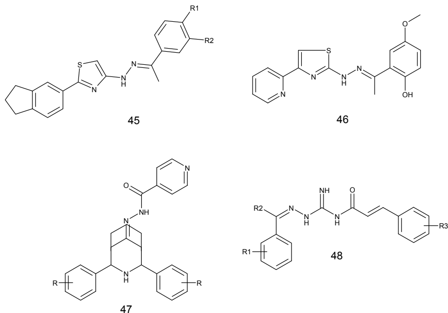
Fig. 14. Hydrazone derivatives as anti-TB agents.
