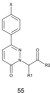
Fig. 18. N -substituted-pyridazinones derivatives.
