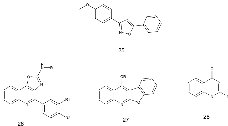
Fig. 7. Quinoline and oxazole derivatives as anti-TB agents.
