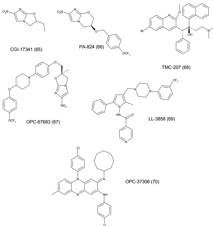
Fig. 25. Anti TB compounds in clinical trials.
