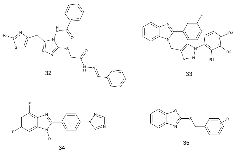
Fig. 9. Triazole and benzimidazole scaffold for designing new anti-TB agents.
