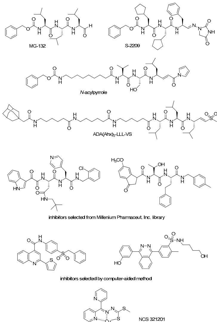
Fig. 20. Structurally diverse, synthetic inhibitors of proteasome.
