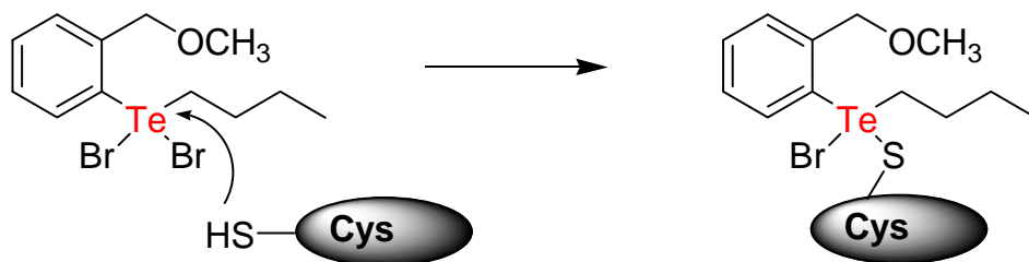
Fig. 10. Mechanism of irreversible inhibition of cathepsins by organotellurane.
