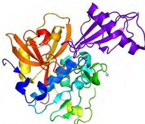
Fig. 1. Stefin A (violet) complexed with cathepsinB.
