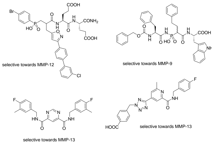
Fig. 23. Selective MMP inhibitors.
