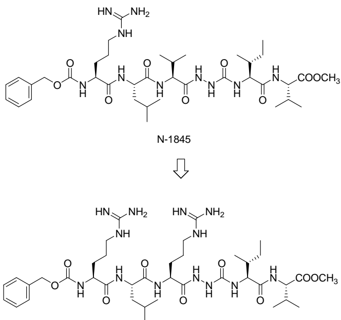
Fig. 2. Two potent azapeptide inhibitors of cathepsin B.
