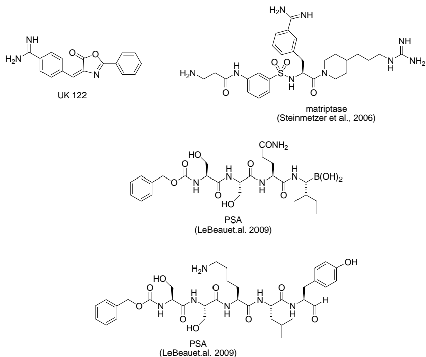
Fig. 16. Representative examples of reversible inhibitors of serine proteinases.
