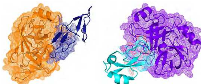
Fig. 11. The binding modes of Bowman-Birk inhibitor with \beta -chymotrypsin (left-hand side) and textilinin with trypsin
