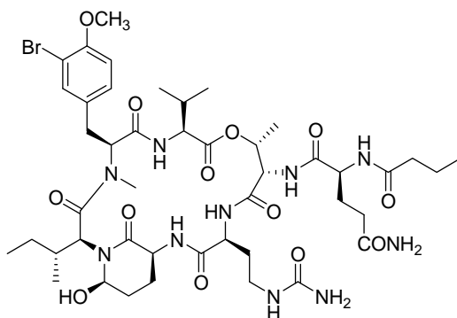
Fig. 13. Structure of Symplocamine A
