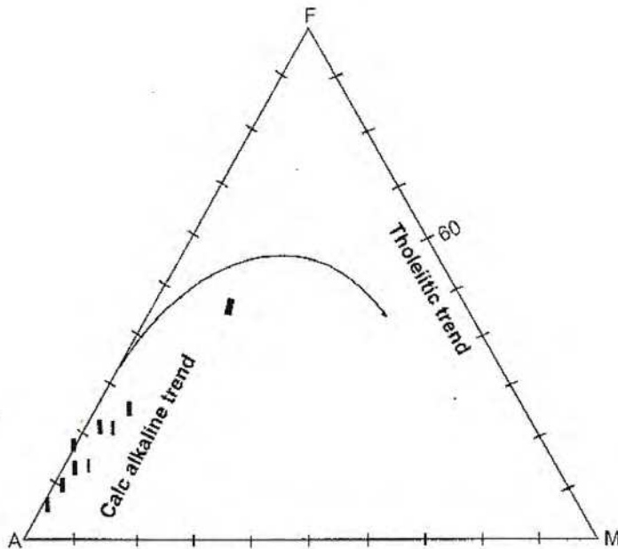
Fig. 2. A= \text{Al}_2\text{O}_3 ; F= \text{FeO} (total iron); M= \text{MgO} (AFM) diagram for the biotite granite gneiss, from Ilesha area
