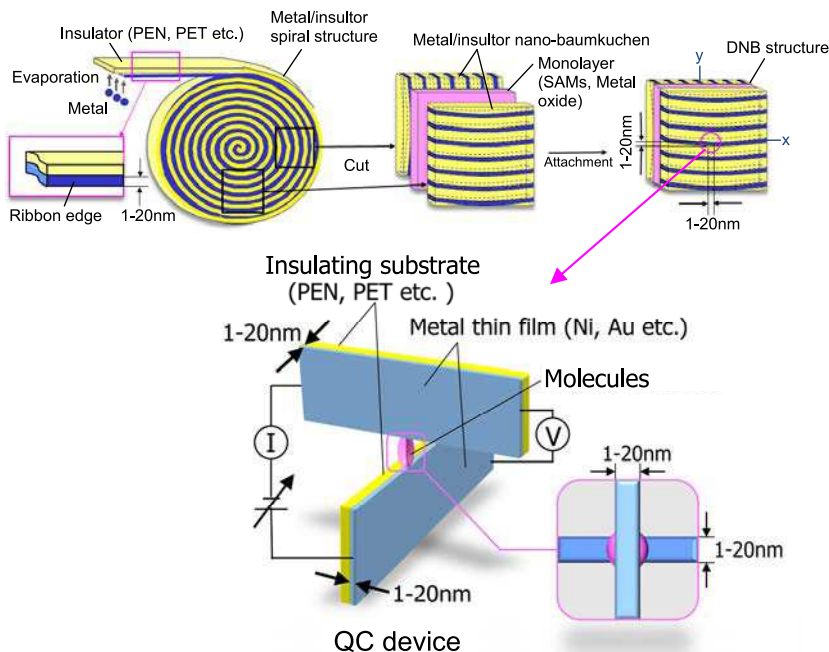
Fig. 1. Fabrication procedure of DNB structures and a schematic illustration of QC devices.
