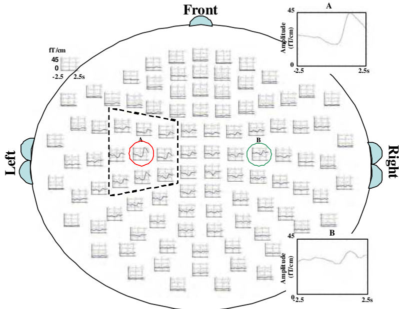
Fig. 6. Sensor-array display of VAMW_{recon} s and VAMW s. (a) One example of ICA single-trial VAMW_{recon} s of all sensor sites in subject I. The single-trial result shows only left sensorimotor area dominance of event-related activities, as the present study focuses on the area contralateral to movement side and only the left spatial template is used. The dashed trapezoid marks the nine SMI vicinal sensor sites and the VAMW_{recon\_max} is marked with the red circle. (b) Trial-specific frequency band used for VAMW_{recon} s calculation in Fig. 6a. (c) VAMW s obtained from the conventional averaging method over 100 trials in subject I. This figure shows a bilateral beta rebound pattern with contralateral (left hemisphere) dominance.
