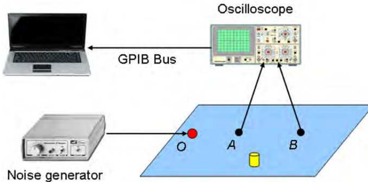
Fig. 11. Experimental set-up for defect detection.
