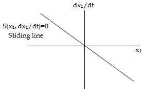
Fig. 4. A prescribed sliding line in phase plane.
