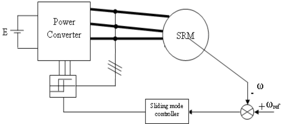
Fig. 2. Control of SRM.
