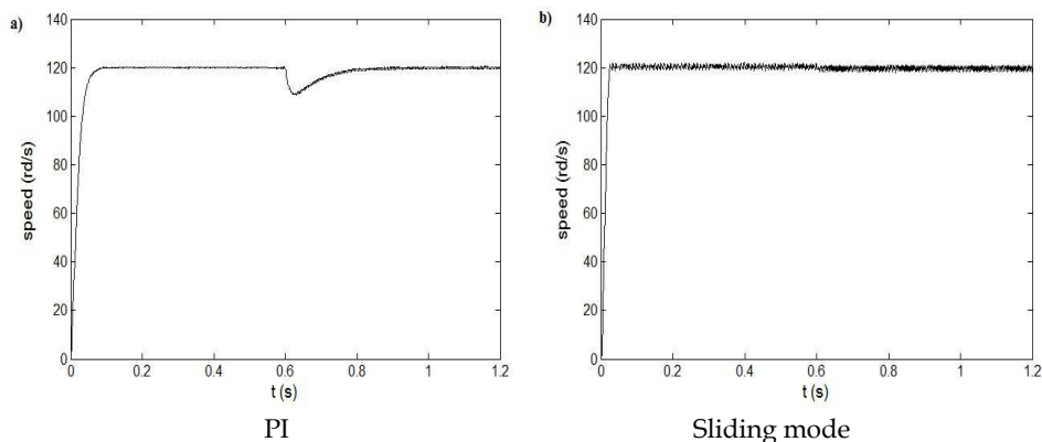
Fig. 5. PI and sliding speed regulation with T_l = 1,5Nm applied at t = 0,6s .
