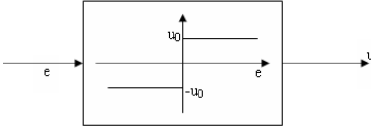
Fig. 3. Relay control.
