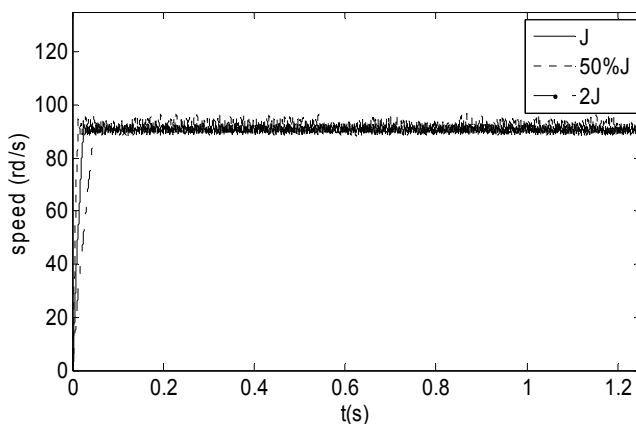
b) Different values of moment of inertia
