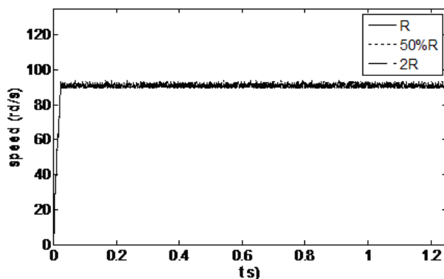
a) Different values of resistance of stator
