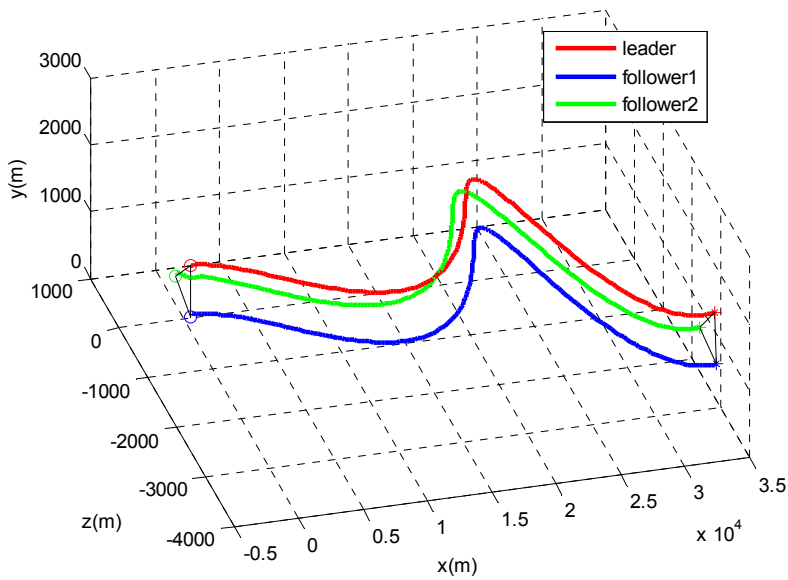
Fig. 13. Three-dimensional trajectories of missile formation under optimal controlling.
