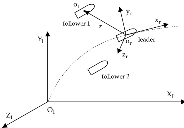
Fig. 4. Relationship between relative and inertial coordinate frame.
