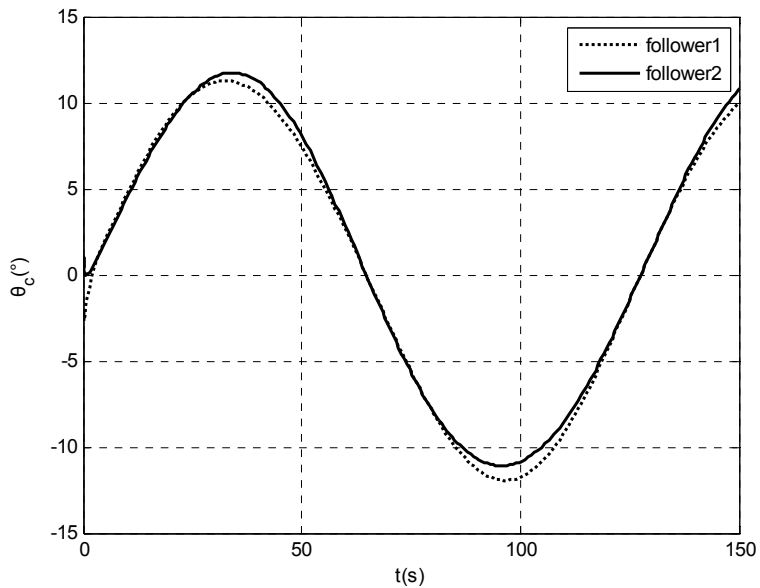
Fig. 11. Flight path angle commands of followers.
