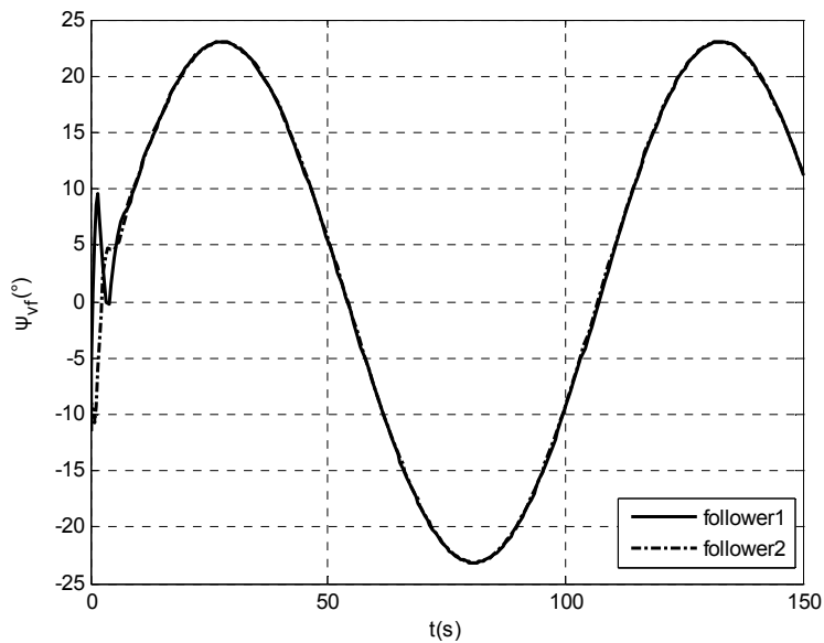
Fig. 18. Flight deflection angle commands of followers.
