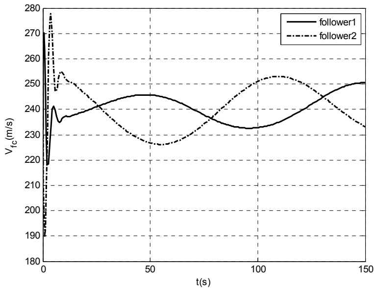
Fig. 16. Velocity commands of followers.
