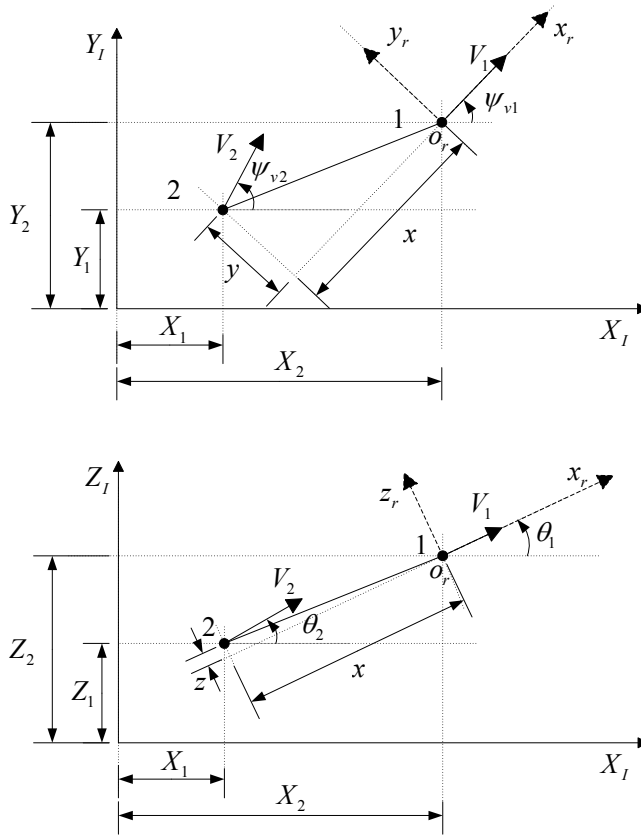
Fig. 5. Relative position relations between two missiles.
