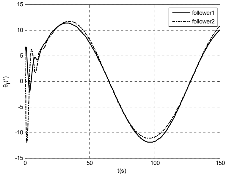
Fig. 17. Flight path angle commands of followers.
