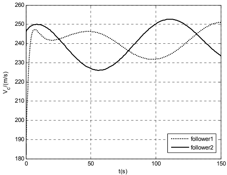
Fig. 10. Velocity commands of followers.
