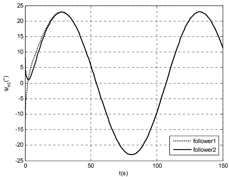
Fig. 12. Flight deflection angle commands of followers.
