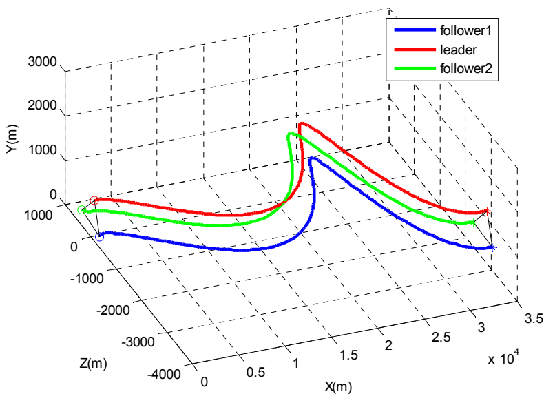
Fig. 6. Three-dimensional trajectories of missile formation under PD controlling.
