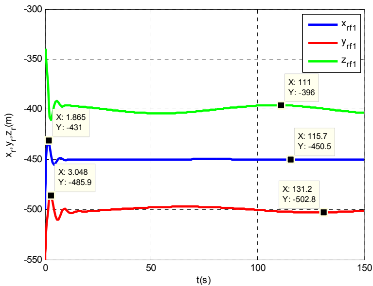
Fig. 14. Distances between follower 1 and leader in relative coordinate frame.
